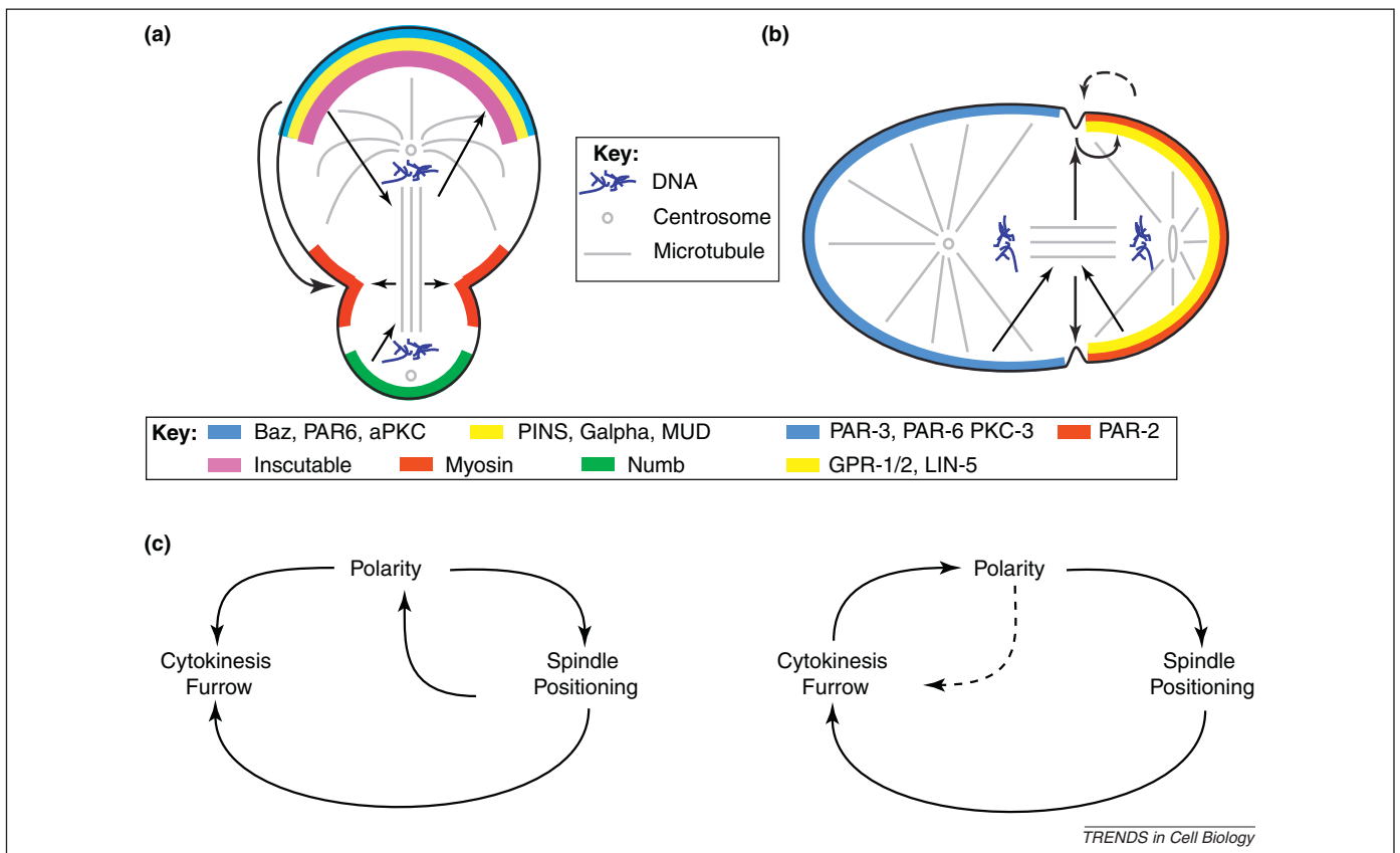
Figure 3. Crosstalk between cell polarity, spindle positioning and cytokinesis furrow ingression. (a) Drosophila neuroblasts are polarized, with Baz, PAR6 and aPKC complex (blue), PINS, G\alpha and MUD (yellow), and Inscuteable (pink) at the apical cortex and Numb (green) at the basal cortex. Cortical polarity controls the position of the mitotic spindle via PINS (arrow from the apical crescent to the spindle), which in turn dictates the position of furrow ingression. In the absence of a mitotic spindle, PINS can asymmetrically position myosin (red) for asymmetric cell division (arrow from the apical crescent to myosin at the furrow ingression). If an axis of polarity is not properly established, interaction of the mitotic spindle with the cortex allows the correct localization of PINS and G\alpha in a mechanism referred to as telophase rescue (arrow from the spindle to the apical crescent). (b) The one-cell C. elegans embryo is polarized, with PAR-3, PAR-6 and PKC-3 at the anterior (blue) and PAR-2 (red) at the posterior. PAR polarity controls the asymmetric enrichment of GPR-1/2 and LIN-5 (yellow) at the posterior. G\alpha , GPR-1/2 and LIN-5 position the spindle, which determines the site of cytokinesis furrow ingression (arrows from the spindle to furrow ingression). In cells where the PAR domain length is altered, the cytokinesis furrow, via G\alpha , can reposition the PAR domain to match the site of cell division (arrow from furrow to polarity). In C. elegans , neuroblast polarity asymmetrically positions myosin for polarized division. Whether this is true in the embryo is unknown (dotted line). (c) Schematic representation of the crosstalk between polarity, spindle positioning and furrow positioning.
