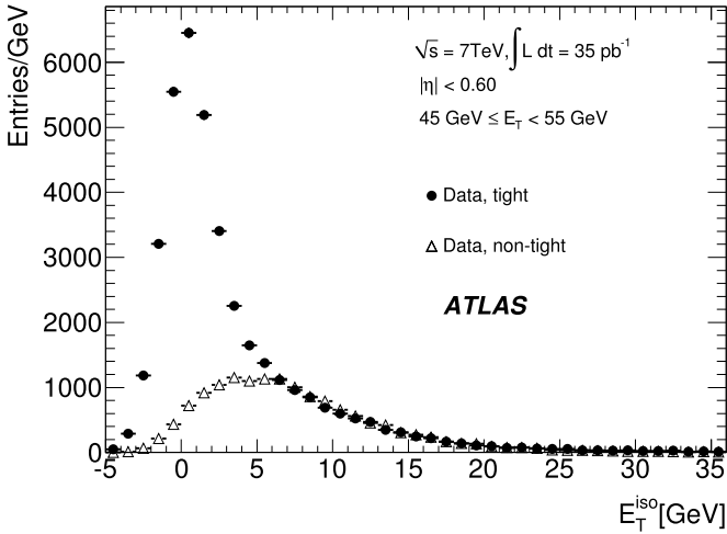
Fig. 1. Distributions of E_T^{\text{iso}} for photon candidates with 45 < E_T < 55 GeV in |\eta| < 0.6 passing the tight (solid dots) and non-tight (open triangles) shower-shape-based selection criteria. The non-tight distribution is normalized to the tight distribution for E_T^{\text{iso}} > 5 GeV (non-isolated region), where the signal contamination is fairly small.
