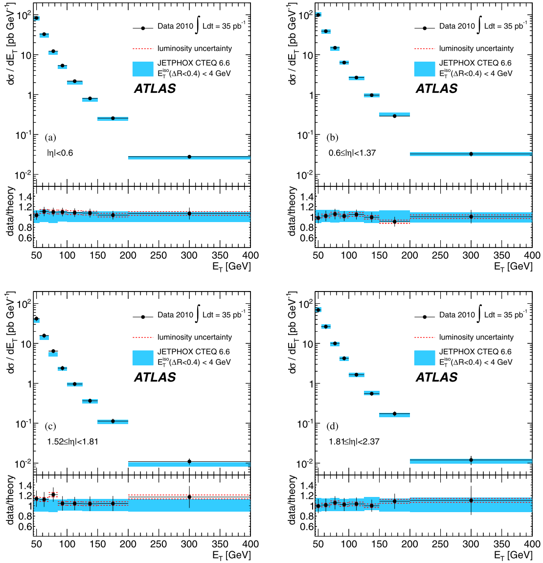
Fig. 2. Measured (dots) and expected (shaded area) inclusive prompt photon production cross-sections, and their ratio, as a function of the photon E_T and in the range (a) |\eta| < 0.6 , (b) 0.6 \leq |\eta| < 1.37 , (c) 1.52 \leq |\eta| < 1.81 and (d) 1.81 \leq |\eta| < 2.37 . The data error bars combine the statistical and systematic uncertainties, with the luminosity uncertainty shown separately (dotted bands).
