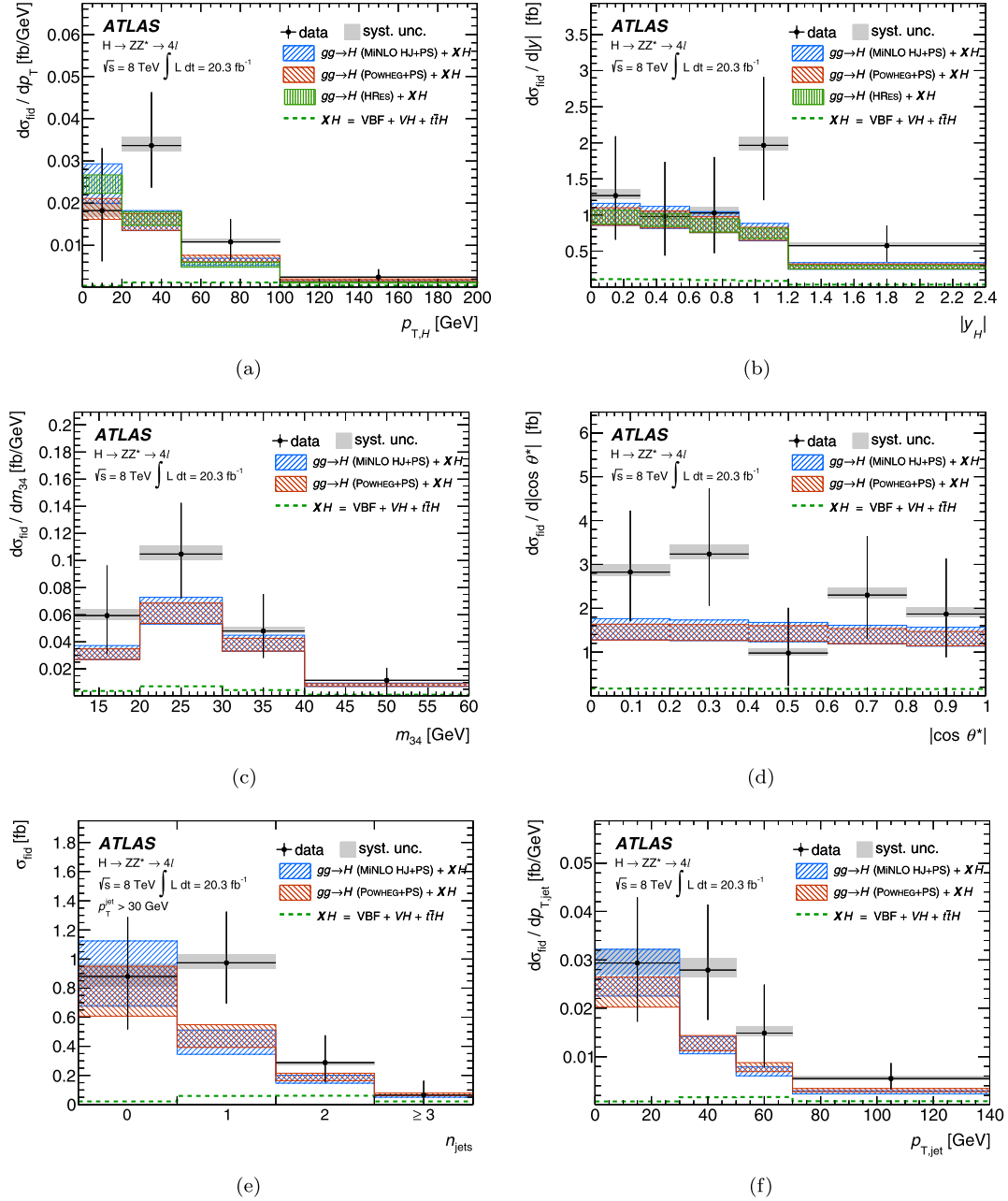
Fig. 2. Differential unfolded cross sections for the transverse momentum p_{T,H} and rapidity y_H of the Higgs boson, the invariant mass of the subleading lepton pair m_{34} , the magnitude of the cosine of the decay angle of the leading lepton pair in the four-lepton rest frame with respect to the beam axis |\cos\theta^*| , the number of jets n_{\text{jets}} , and the transverse momentum of the leading jet p_{T,\text{jet}} in the H \rightarrow ZZ^* \rightarrow 4\ell decay channel compared to different theoretical calculations of the ggF process: POWHEG, MINLO and HRES2. The contributions from VBF, ZH/WH and t\bar{t}H are determined as described in Section 2 and added to the ggF distributions. All theoretical calculations are normalized to the most precise SM inclusive cross-section predictions currently available [60]. The error bars on the data points show the total (stat. \oplus syst.) uncertainty, while the grey bands denote the systematic uncertainties. The bands of the theoretical prediction indicate the total uncertainty. (For interpretation of the references to colour in this figure legend, the reader is referred to the web version of this article.)
