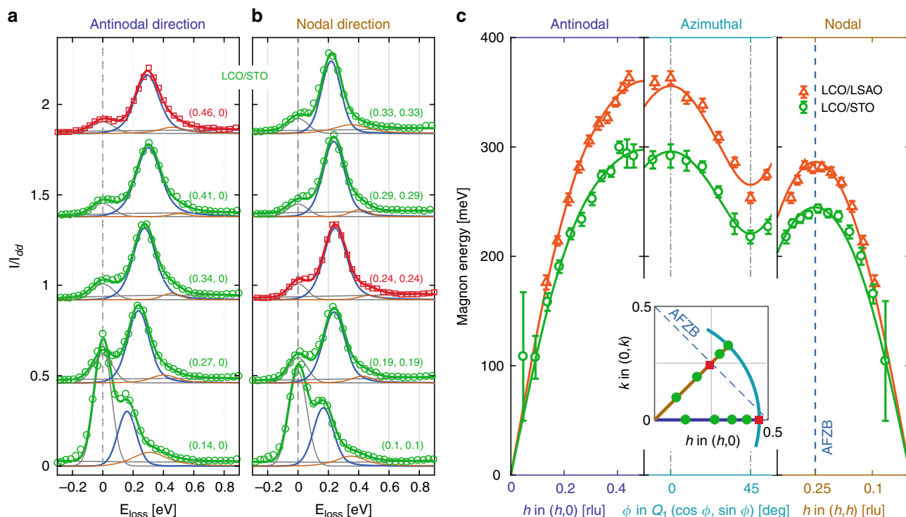
Fig. 2 Magnon dispersions of \text{La}_2\text{CuO}_4 thin films. a , b display raw RIXS spectra recorded on the LCO/STO thin film system, along the antinodal [1\ 0] and nodal [1\ 1] directions, respectively. Red curves represent the data close to the antiferromagnetic zone boundary (AFZB) as shown in the inset in c . Solid lines are fits to the data (see text for detailed description). Notice that elastic scattering is, as expected, enhanced as the specular condition (0,0) is approached. In (c) magnon dispersions of LCO/LSAO and LCO/STO, extracted from fits to raw spectra as in a , b , along three different momentum trajectories (see solid lines in the inset) are presented. Solid lines through the data points are obtained from two-dimensional fits using Hubbard model (see the main text). Error bars are three times the standard deviations extracted from the fits. In (c) Q_1 takes different values for each compound due to slightly different incident energies and in-plane lattice parameters, resulting in 0.4437 (0.4611) for LCO/LSAO (LCO/STO). Source data are provided as a Source Data file
