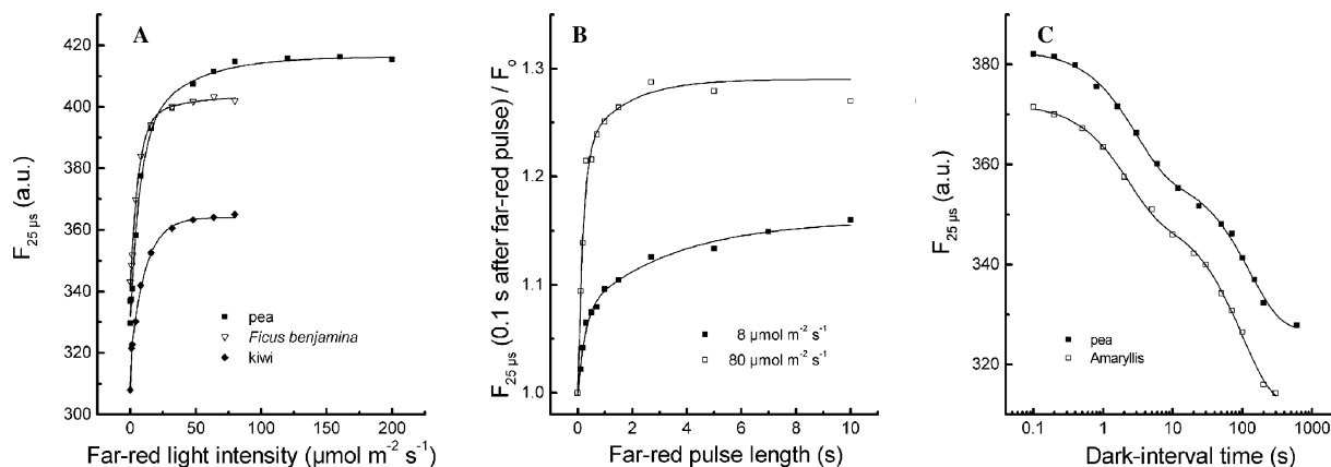
Figure 2. Light and dark-adaptation of the F_{25\ \mu\text{s}} -level as a function of a far-red pre-illumination. In (A) and (B) far-red-light-dose response curves are shown. The dose was varied either by changing the far-red light intensity (A) or by changing the pulse length (B). In (C) the F_{25\ \mu\text{s}} -level as a function of the dark-time interval after a 10 s 80\ \mu\text{mol m}^{-2}\text{s}^{-1} far-red light pulse is shown. The F_{25\ \mu\text{s}} -levels in (A) and (B) were determined 100 ms after the far-red pre-illumination. The far-red pulse length in (A) and (C) was 10 s. In (B) only data obtained from pea leaves are shown. For the different panels data from 3–5 independent measurements were averaged.
