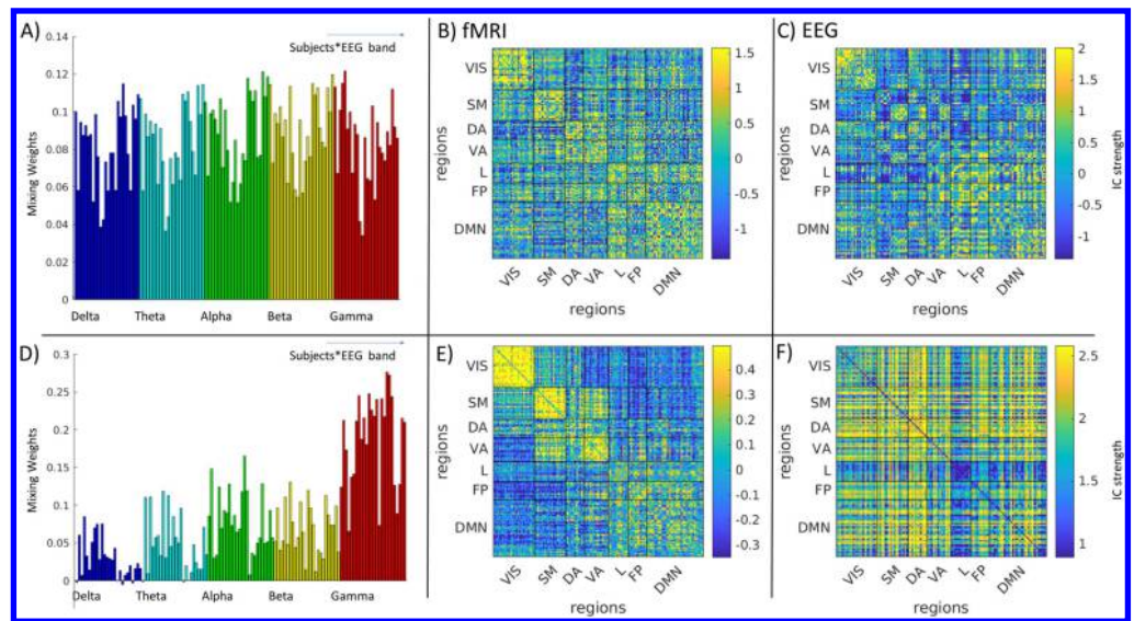
Figure 4. (A) Subject- and band-specific mixing weights of the hybrid EEG-fMRI ICN-FG component. (B) fMRI part of the ICN-FG component. (C) EEG part of the ICN-FG component. Note that as we stacked up all frequency-specific EEG connectomes for each subject (cf. Figure 2), we obtained a single EEG component part (C) associated with an ICA mixing weight for each subject and frequency (represented by one bar each in A). (D–F) These panels visualize equivalent aspects for the VIS-FS component. All panels represent the main dataset (for generalization data see Supporting Information Figure S3. Colorbars have been saturated at 95th and 5th percentile for better comparison with Figures 5 and 6). VIS = visual; SM = somatomotor; DA = dorsal attention; VA = ventral attention; L = limbic; FP = fronto-parietal; DMN = default mode network.
