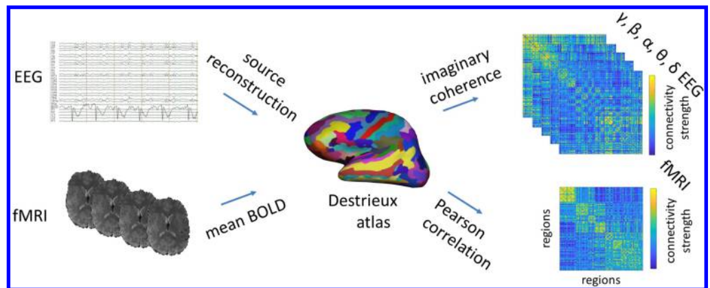
Figure 1. Construction of EEG and fMRI connectomes. EEG and fMRI data were parcellated into the 148 cortical regions of the Destrieux atlas as follows. EEG was source reconstructed to a fine-grained grid, and the time courses of the solution points were averaged per region and per subject. For fMRI, the BOLD signal time course was averaged over the voxels in each region for each subject. Pearson correlation of the mean fMRI-BOLD time courses and imaginary part of the coherency of averaged EEG source signals were used to build functional connectivity matrices/connectomes ( FC_{EEG} and FC_{fMRI} ) for each subject.
