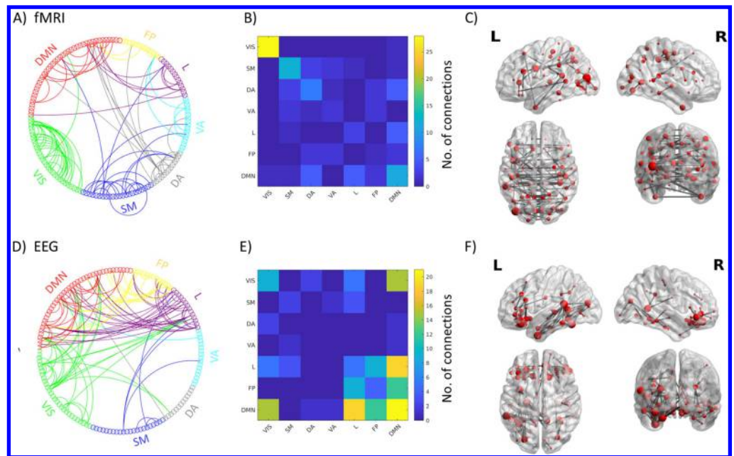
Figure 5. Connections with highest nodal strength (99th percentile) for the ICN-FG component: circle graphs show all connections between different ICN networks for fMRI (A) and EEG (D); matrices summarize the number of connections falling into each ICN-ICN pair for fMRI (B) and EEG (E); brain renderings show strongest connections of the components on a canonical reconstructed cortical surface for the fMRI (C) and EEG (F) part of the hybrid component. Data correspond to the main dataset; for the results of the generalization dataset see Supporting Information Figure S4. VIS = visual; SM = somatomotor; DA = dorsal attention; VA = ventral attention; L = limbic; FP = fronto-parietal; DMN = default mode network.
