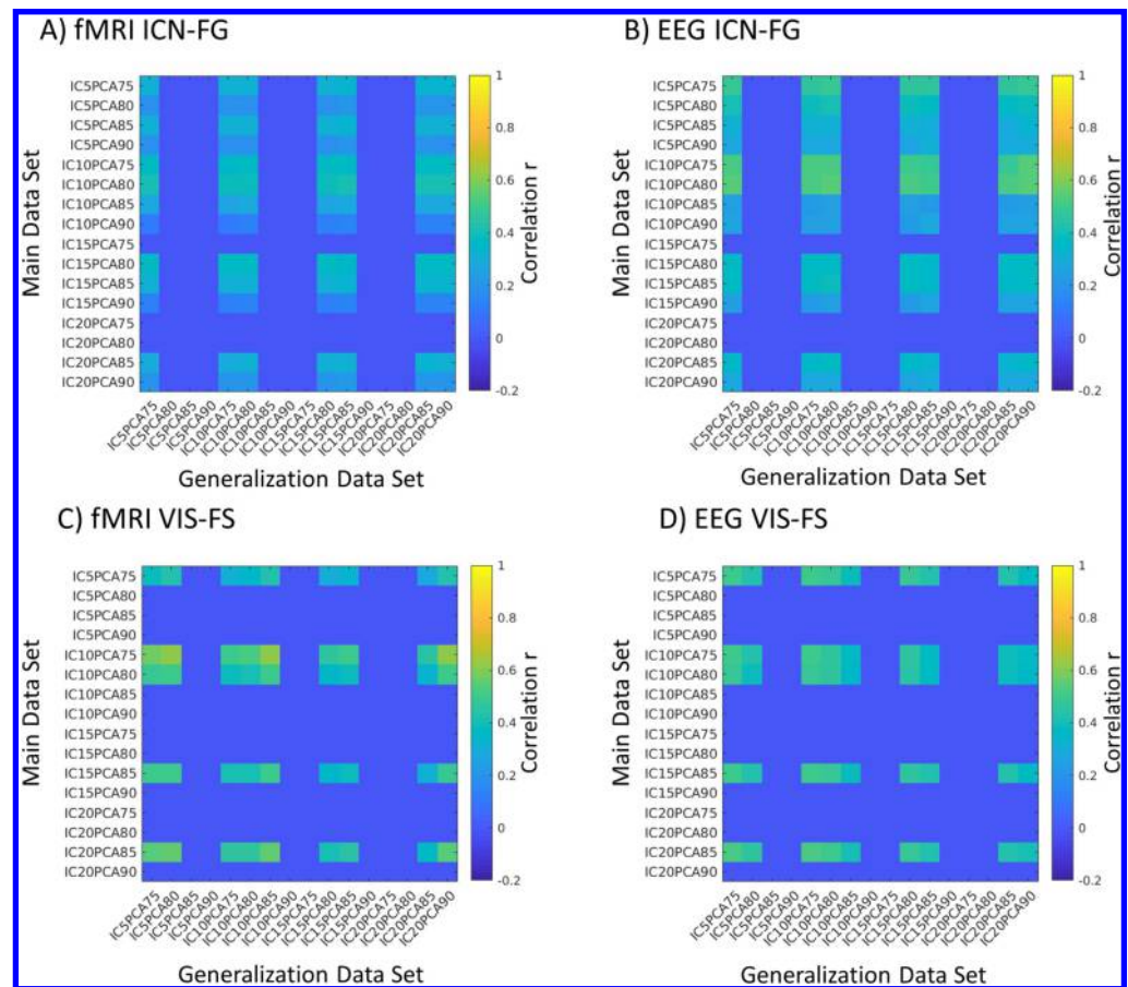
Figure 3. Impact of the choice of free parameters on the consistency across datasets. Matrices visualize the intercorrelation between the IC strengths of the two datasets by using different parameter sets, shown separately for the EEG and fMRI parts of the ICN-FG and VIS-FS components (A–D). We tested all combinations, keeping principal components with 75–90% of the variance, followed by an independent component analysis keeping 5–20 ICs (e.g., IC5PCA75 depicts an analysis using 5 ICs and keeping all PCs that cumulatively explain 75% of the data variance). Rows with consistent correlation of zero mean that in one of the datasets, the preceding separate ICC procedure had found no component passing stability requirements for this parameter combination. There is significant ( p < 10^{-100} ) spatial correlation of IC matrices between datasets for all parameters for which stable ICs had been identified (average correlation for the ICN-FG component: fMRI part r = 0.27 ; EEG part r = 0.35 ; and for the VIS-FS component: fMRI part r = 0.45 ; EEG part r = 0.44 ).
