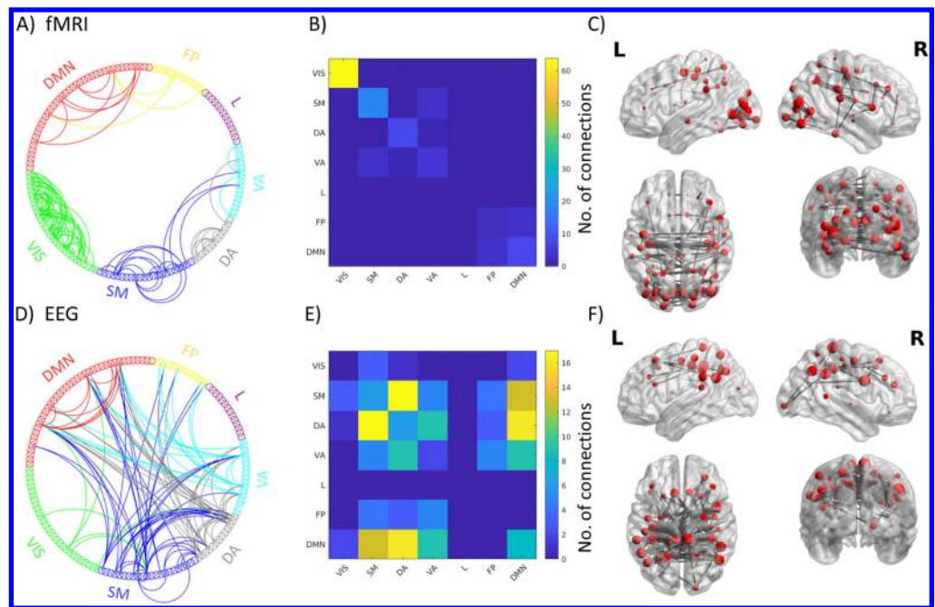
Figure 6. Connections with highest nodal strength (99th percentile) for the VIS-FS component: circle graphs show all connections between different ICN networks for fMRI (A) and EEG (D); matrices summarize the number of connections falling into each ICN-ICN pair for fMRI (B) and EEG (E); brain renderings show strongest connections of the components on a canonical reconstructed cortical surface for the fMRI (C) and EEG (F) part of the hybrid component. Data correspond to the main dataset; for the results of the generalization dataset see Supporting Information Figure S5. VIS = visual; SM = somatomotor; DA = dorsal attention; VA = ventral attention; L = limbic; FP = fronto-parietal; DMN = default mode network.
