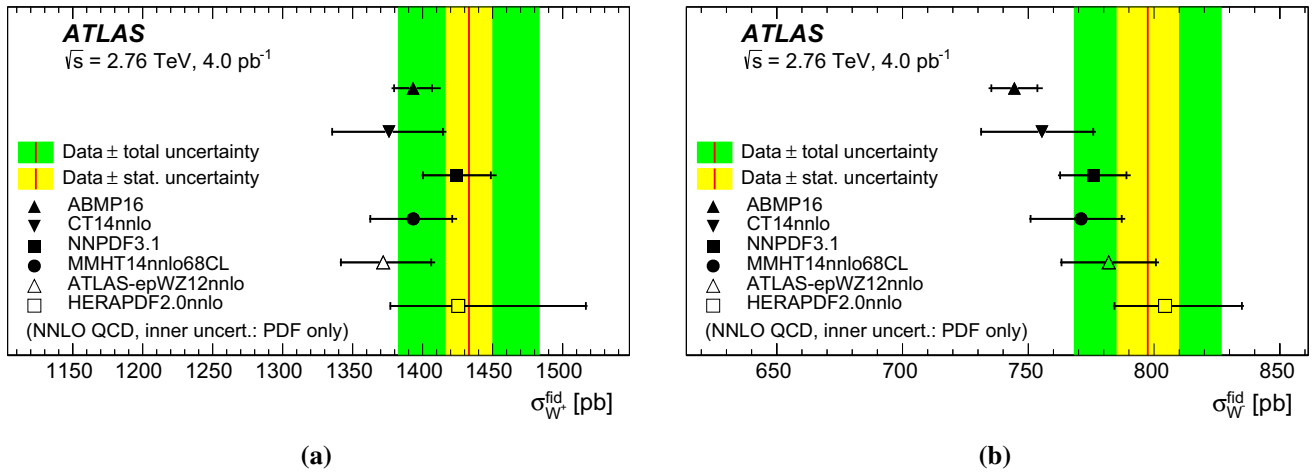
Fig. 5 NNLO predictions for the fiducial cross-section (a) \sigma_{W^+}^{\text{fid}} and (b) \sigma_{W^-}^{\text{fid}} for the six PDFs CT14nnlo, MMHT2014, NNPDF3.1, ATLASepWZ12, ABMP16 and HERApdf2.0 compared with the measured fiducial cross-section as given in Table 7. The inner shaded band
