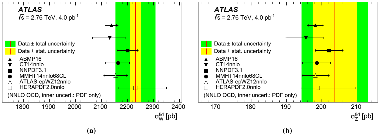
Fig. 6 NNLO predictions for the fiducial cross-sections (a) \sigma_{W^+}^{\text{fid}} and (b) \sigma_Z^{\text{fid}} for the six PDFs CT14nnlo, MMHT2014, NNPDF3.1, ATLASepWZ12, ABMP16 and HERApdf2.0 compared with the measured fiducial cross-section as given in Table 7. The inner shaded band
