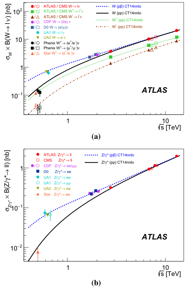
Fig. 4 The measured values of (a) \sigma_W \times B(W \rightarrow \ell \nu) for W^+ bosons, W^- bosons and their sum and (b) \sigma_{Z/\gamma^*} \times B(Z/\gamma^* \rightarrow \ell\ell) for proton–proton and proton–antiproton collisions as a function of \sqrt{s} . Data points at the same \sqrt{s} are staggered to improve readability. All data points are shown together with their total uncertainty. The theoretical calculations are performed at NNLO in QCD using DYNLLO 1.5 and FEWZ 3.1 as described in the text. The theoretical uncertainties are not shown
