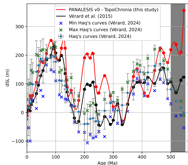
Figure 5. Sea-level (black) from V  rard et al. (2015) and PANALEISIS v0 using TopoChronia (red) compared to Haq's curves values from V  rard (2024). The data have been resampled to match PANALEISIS reconstruction intervals (horizontal error bars). Vertical error bars represent the two sigma errors calculated from all values within each time interval. Green and blue crosses indicate the maximum and minimum values of Haq's curves within each interval.
