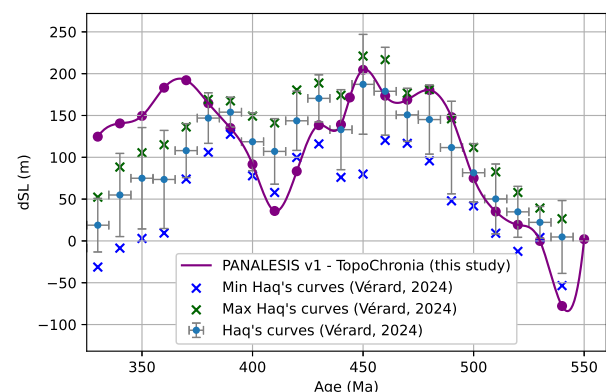
Figure 6. Sea-level (purple) PANALEISIS v1 curve using TopoChronia compared to Haq's curves values from V  rard (2024). Same legend as in Figure 5.
