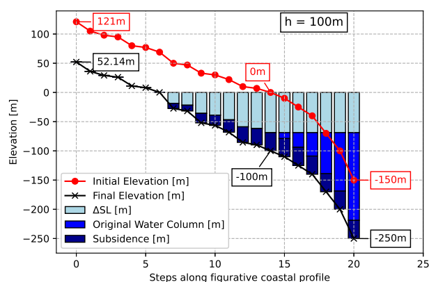
Figure 7. Figurative coastal profile water load correction example, for an added water column height ( h ) of 100m, \Delta SL of \approx 69 m (light blue) and subsidence ( S ) of \approx 31 m (dark blue). The original water column (regular blue) corresponds to the initial elevation, and applies only for points originally under water (initial elevation < 0 m).
