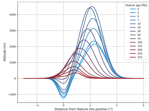
Figure 1. Example of synthetic elevation associated with a collision zone, evolving alongside a profile that is perpendicular to the original collision line. Elevation is controlled by the feature age and by the distance from the original feature line.
