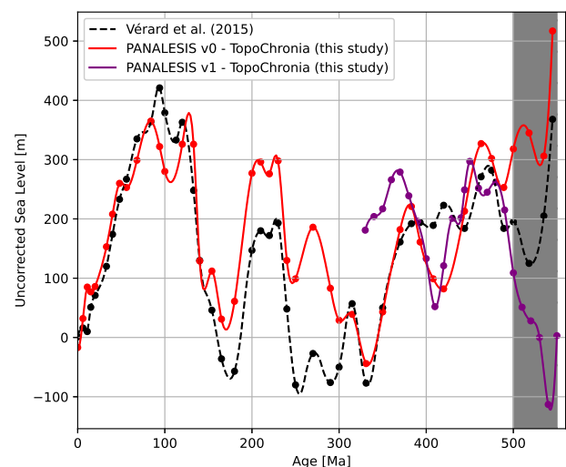
Figure 3. Uncorrected sea-level [m] using PANALEISIS v0 and v1 for the Phanerozoic. In black, original results Vérard et al. (2015), in red and purple, new results using TopoChronia on PANALEISIS v0 and v1, respectively. Dark grey area indicates time ranges for which the PANALEISIS v0 and UNIL model do not cover 100% of the Earth surface, PANALEISIS v1, under construction, covers 100% back to 750 Ma.
