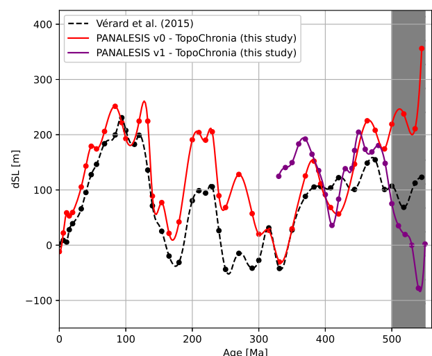
Figure 4. Corrected sea-level [m] performance of PANALEISIS v0 and v1 for the Phanerozoic. Same legend as for Figure 3.
