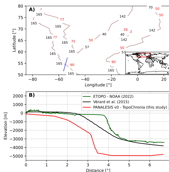
Figure 8. A) Example of discrepancies in feature ages of passive margins from the PANALEISIS v0 model present-day reconstruction (grey lines). Values in black are the ages defined in the UNIL model and used in V  rard et al. (2015), while ages in red are ages defined in the PANALEISIS v0 model and used for TopoChronia. The blue line represents a profile for which we measured the elevation, shown in B).
