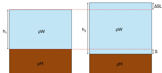
Figure 2. Water load correction according to Airy's model, modified after Allen and Allen (2005). The added water column is divided into an extra height of water above initial level ( \Delta SL ) and subsidence of the oceanic floor ( S ).
