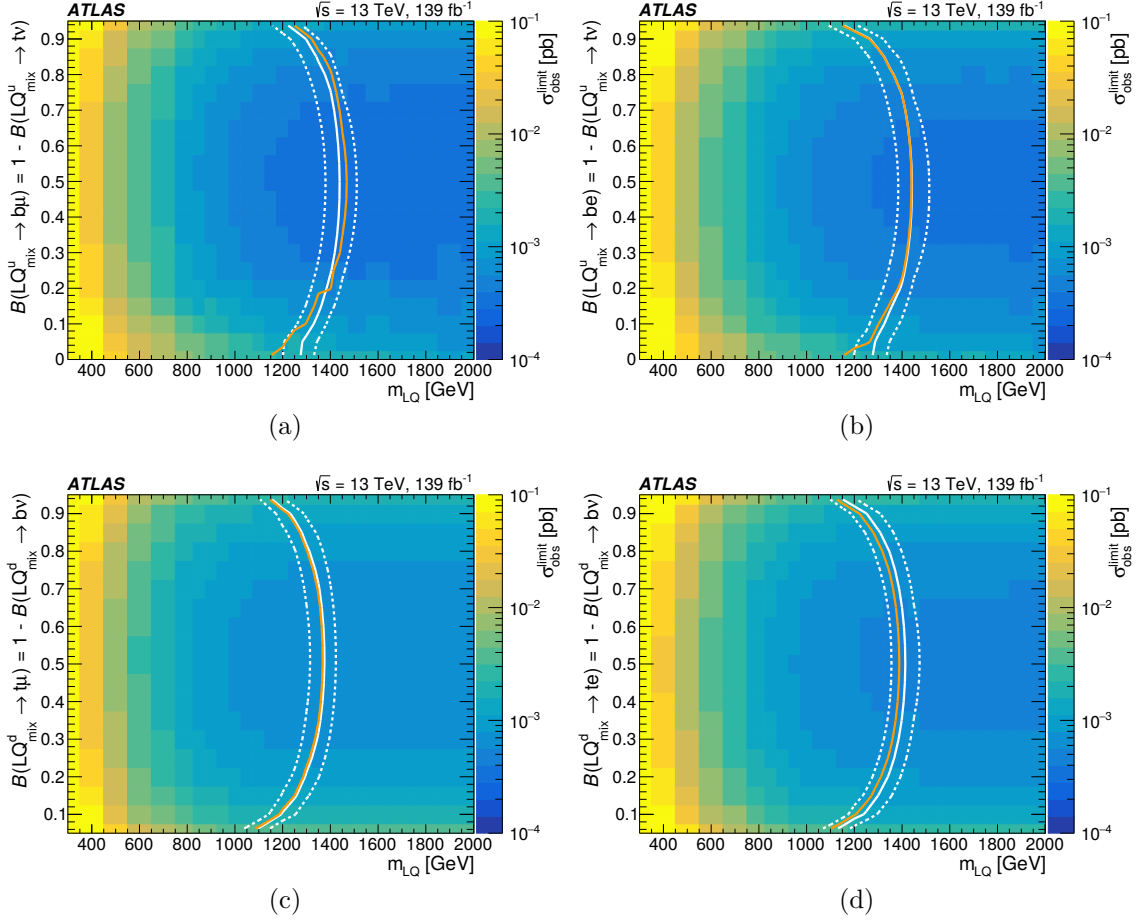
Figure 9. Expected (solid white, \pm 1\sigma ranges dashed) and observed (solid orange) exclusion limits on the leptoquark mass as a function of the branching ratio into charged leptons at 95 % CL. The observed upper limit on the signal cross-section in each bin is shown on the z-axis. Limits are presented for (a) up-type scalar LQs decaying into muons, (b) up-type scalar LQs decaying into electrons, (c) down-type scalar LQs decaying into muons, and (d) down-type scalar LQs decaying into electrons. For up-type LQs the range in \mathcal{B} is 0–0.95, for down-type it is 0.05–0.95.
