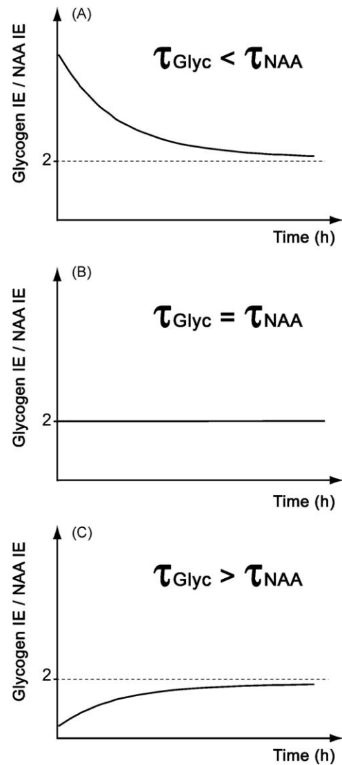
Fig. 2. The 3 different curves that could be obtained by plotting Glyc IE/NAA IE over time using Eq. (4). These curves depend on the values of \tau_{Glyc} and \tau_{NAA} . The 3 different case figures are shown in (A) if \tau_{Glyc} < \tau_{NAA} , in (B) if \tau_{Glyc} = \tau_{NAA} or in (C) if \tau_{Glyc} > \tau_{NAA} .
