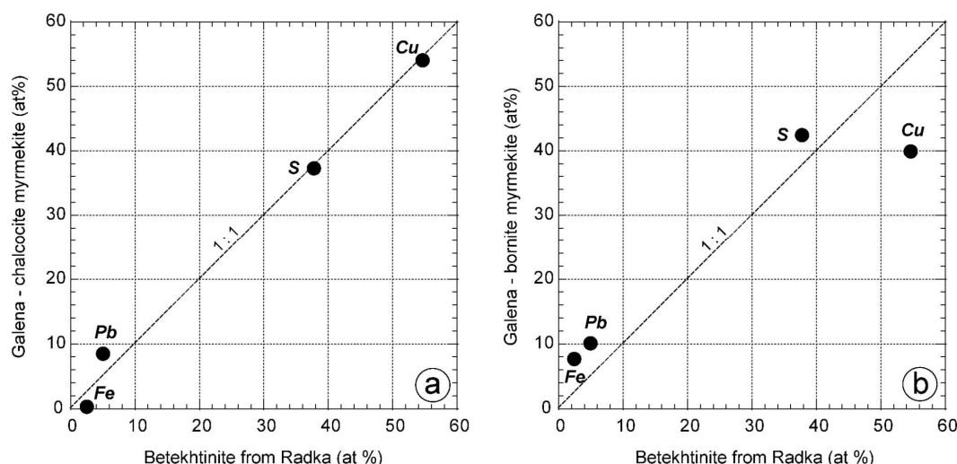
Fig. 6. Projection of the betekhtinite composition from Radka versus composition of symplectites (at%). Concentrations are based on image analysis results, taking in account the average compositions of galena, chalcocite and bornite from Radka (Table 2). Betekhtinite composition is based on electron microprobe analyses (Table 3): a) Galena-chalcocite symplectite; b) Galena-bornite symplectite
