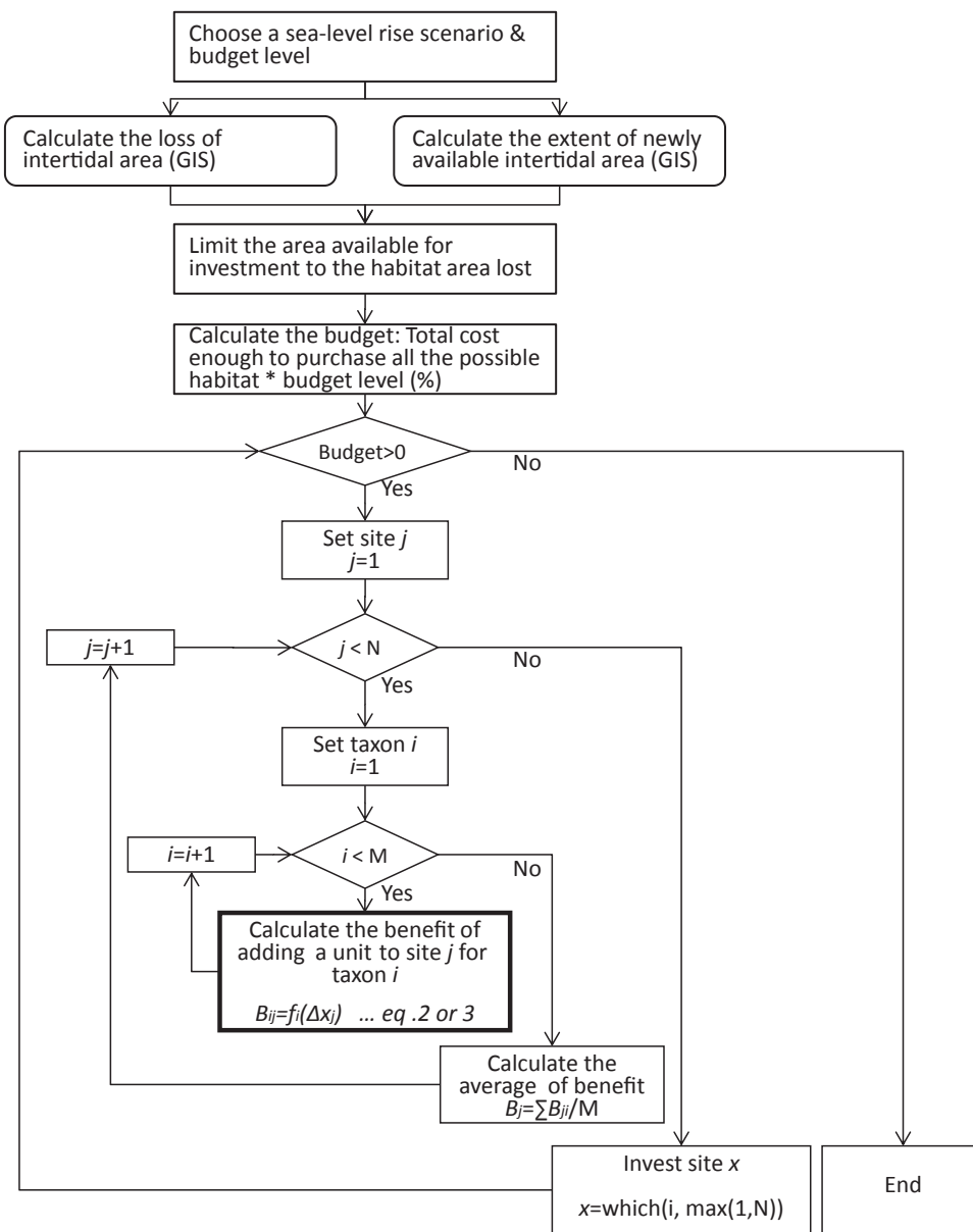
Figure 1. Resource allocation algorithm of the flyway strategy for conserving migratory shorebirds in East Asian-Australasian Flyway (N, total number of sites, in this case 163; M, number of taxa, in this case 10; \Delta x_j , investment in site j). Investment is allocated to maximize average population persistence across the 10 taxa. The investment is repeated until the budget is consumed. The rectangle with a heavy line is the calculation of the benefit of investment.
