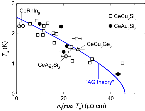
Fig. 4 Pair-breaking systematics: T_c vs \rho_0 ( \rho_0 taken at the pressure of maximal T_c ) of the \text{CeCu}_2\text{Si}_2 family and \text{CeRhIn}_5 (published and unpublished data, see Supplementary Fig. S1 for references). The error bars on \rho_0 result from the power-law extrapolation to zero temperature of \rho(T) . The solid line represents the generalized Abrikosov-Gor'kov theory with a critical resistivity \rho_0^{\text{cr}} = 46 \mu\Omega\text{cm} 38
