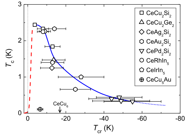
Fig. 5 Building superconductivity up in heavy fermion compounds. The presented T_c -vs- T_{\text{cr}} relation is qualitatively predicted by CVF theory. 23,24 The continuous line is a guide to the eyes. The dashed line represents a qualitative prediction from CVF theory. 23 The error bars on T_{\text{cr}} represent estimated errors according to the scaling analysis (see main text). The arrow indicates T_{\text{cr}} of \text{CeCu}_6 (no SC)
