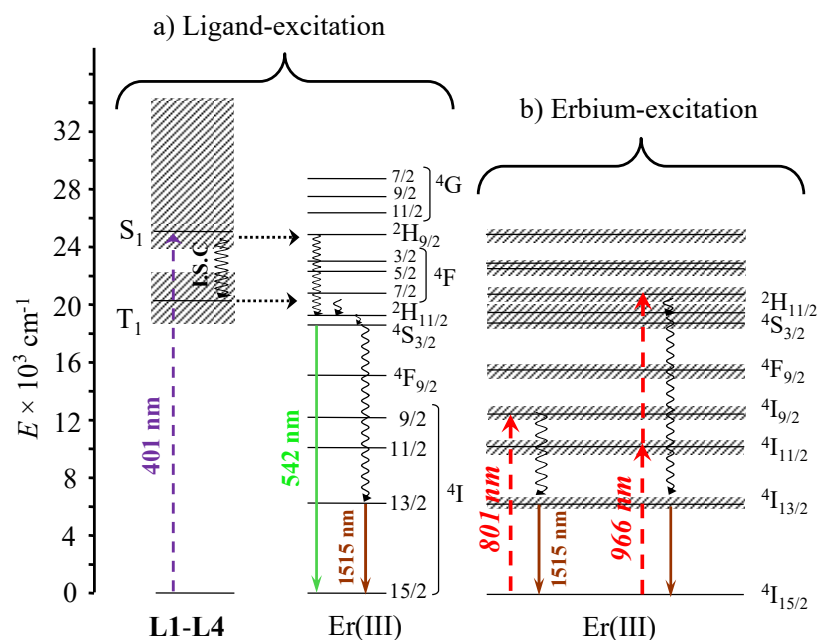
Fig. 4 Jablonski diagram summarizing the downshifting processes following a) ligand-centered or b) erbium-centered excitation (dashed upward arrows), energy transfers (dotted horizontal arrows), non-radiative multiphonon relaxation (undulating arrows) and radiative emission processes (straight downward arrows) operating in the complexes [Er(Lk)_3]^{3+} ( Lk = 1-4 ).
