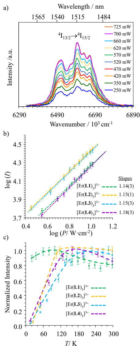
Fig. 5 a) Near-infrared downshifted \text{Er}(^4\text{I}_{13/2} \rightarrow ^4\text{I}_{15/2}) emission observed for [\text{Er}(\text{L1})_3](\text{ClO}_4)_3 in acetonitrile (10 mM, 298 K) upon laser excitation of the \text{Er}(^4\text{I}_{9/2} \leftarrow ^4\text{I}_{15/2}) transition at \lambda_{\text{exc}} = 801 \text{ nm} ( \tilde{\nu}_{\text{exc}} = 12284 \text{ cm}^{-1} ) and for different incident pump intensities focused on a spot size of \approx 0.07 \text{ cm}^2 and b) corresponding log-log plots of downshifted intensities I as a function of incident pump intensities P (in \text{W}\cdot\text{cm}^{-2} ) for [\text{Er}(\text{L}k)_3]^{3+} in acetonitrile (The straight lines correspond to extrapolated linear fits) and c) dependences of downshifted intensities I as a function of temperature (solid state, P = 10 \text{ W}\cdot\text{cm}^{-2} , the dashed lines are only guides for the eyes).
