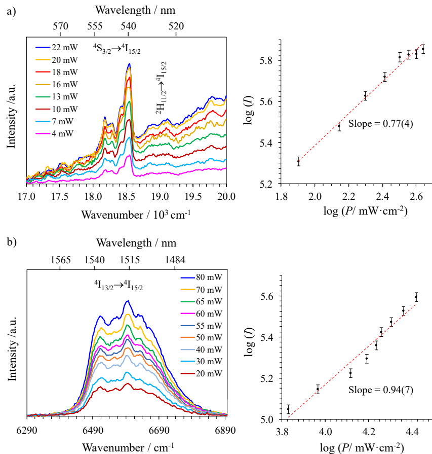
Fig. 3 Downshifted a) visible and b) near-infrared emissions and corresponding log-log plots of downshifted intensities I as a function of incident pump intensities P (in \text{mW}/\text{cm}^2 ) observed for [\text{Er}(\mathbf{L1})_3](\text{ClO}_4)_3 (solid state, 298 K) upon ligand-centered laser excitation at 401 nm ( 24938 \text{ cm}^{-1} ) and for different incident pump intensities focused on a spot size of \approx 0.05 \text{ cm}^2 .
