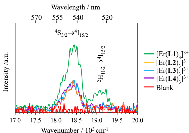
Fig. 8 Upconverted visible \text{Er}(^2\text{H}_{11/2} \rightarrow ^4\text{I}_{15/2}) and \text{Er}(^4\text{S}_{3/2} \rightarrow ^4\text{I}_{15/2}) emissions observed for [\text{Er}(\mathbf{Lk})_3]^{3+} ( \mathbf{Lk} = \mathbf{L1-L4} ) complexes recorded upon laser excitation of the \text{Er}(^4\text{I}_{11/2} \leftarrow ^4\text{I}_{15/2}) transition at \lambda_{\text{exc}} = 966 nm ( \tilde{\nu}_{\text{exc}} = 10350 \text{ cm}^{-1} ) and using incident pump intensity P = 78 \text{ W} \cdot \text{cm}^{-2} in acetonitrile solution ( c \sim 10 \text{ mM} , Table S1) at 298 K. The blank (red curve) was recorded from pure acetonitrile solvent using incident pump intensity P = 78 \text{ W} \cdot \text{cm}^{-2} .
