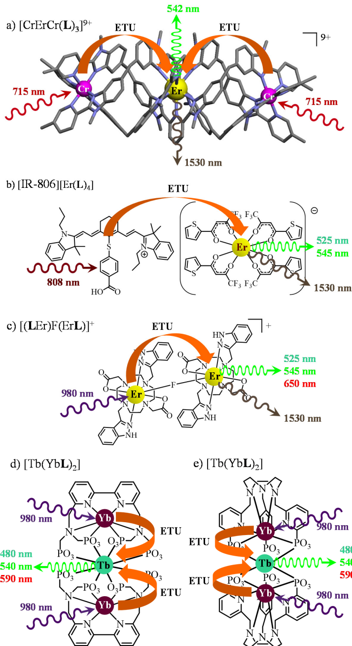
Fig. 1 Erbium-based coordination complexes exhibiting linear upconversion processes following the ETU mechanism. The X-ray crystal structure is shown for a) [\text{CrErCr}(\text{L})_3](\text{CF}_3\text{SO}_3)_9 28a and chemical structures deduced from spectroscopic data recorded in solution are depicted for b) [\text{IR-806}][\text{Er}(\text{L})_4] , 29 c) [(\text{LEr})\text{F}(\text{ErL})]^+ 30 and d),e) [\text{Tb}(\text{YbL})_2] . 31
