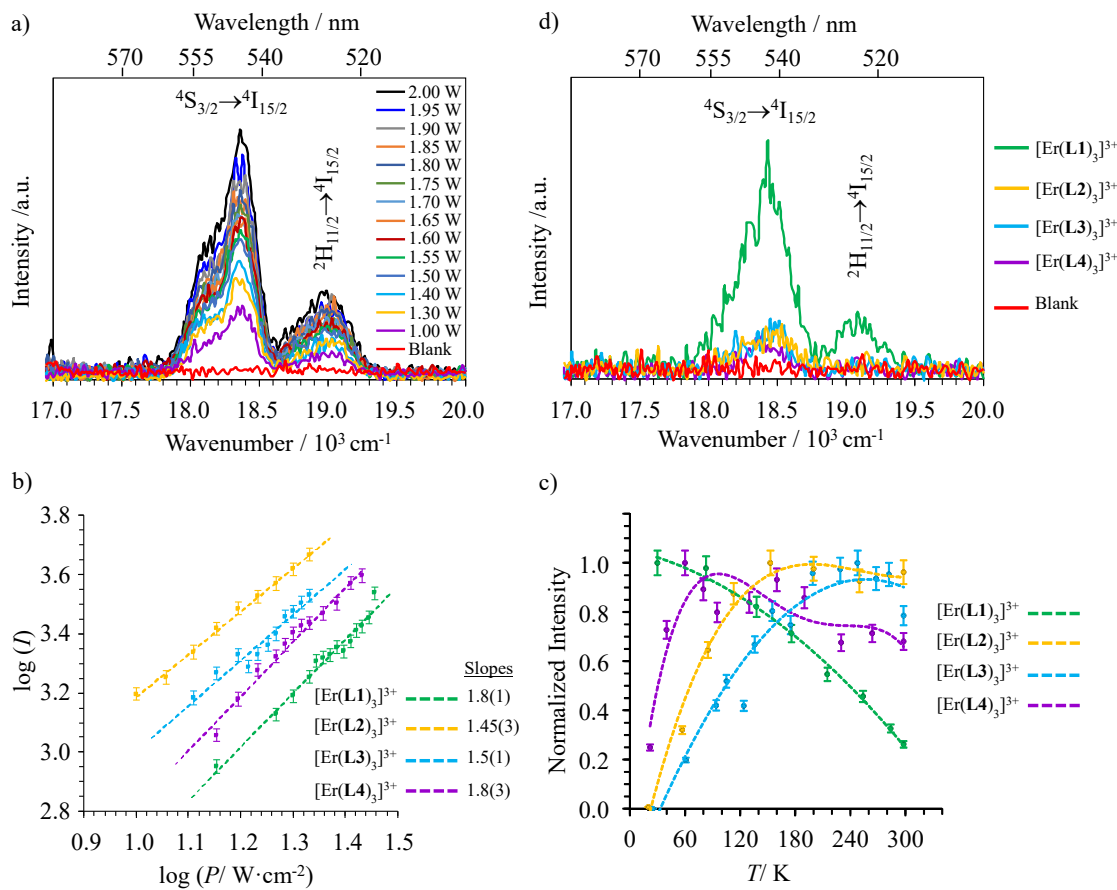
Fig. 6 a) Upconverted visible \text{Er}({}^2\text{H}_{11/2} \rightarrow {}^4\text{I}_{15/2}) and \text{Er}({}^4\text{S}_{3/2} \rightarrow {}^4\text{I}_{15/2}) emissions observed for [\text{Er}(\text{L1})_3](\text{ClO}_4)_3 (solid state, 298 K) recorded upon laser excitation of the \text{Er}({}^4\text{I}_{9/2} \leftarrow {}^4\text{I}_{15/2}) transition at \lambda_{\text{exc}} = 801 \text{ nm} ( \tilde{\nu}_{\text{exc}} = 12284 \text{ cm}^{-1} ) and using increasing incident pump intensities focused on a spot size of \approx 0.07 \text{ cm}^2 (the blank (= red curve) was recorded upon irradiation of the copper plate support covered with silver glue at maximum intensity P = 29 \text{ W} \cdot \text{cm}^{-2} ) and b) corresponding log-log plots of upconverted intensities I as a function of incident pump intensities P (in \text{W} \cdot \text{cm}^{-2} ), the straight lines correspond to extrapolated linear fits. c) Dependences of upconverted intensities I as a function of temperature (solid state, P = 29 \text{ W} \cdot \text{cm}^{-2} , the dashed lines are only guides for the eyes) and d) upconverted emissions for [\text{Er}(\text{Lk})_3]^{3+} ( \text{Lk} = \text{L1-L4} ) complexes recorded using incident pump intensity P = 21 \text{ W} \cdot \text{cm}^{-2} in acetonitrile solution ( c \sim 10 \text{ mM} ). The blank (red curve) was recorded from pure acetonitrile solvent using incident pump intensity P = 21 \text{ W} \cdot \text{cm}^{-2} .
