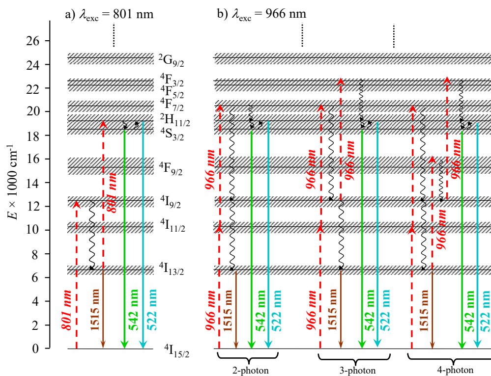
Fig. 7 Jablonski diagram summarizing the mechanisms of the Er-centered upconversion processes operating in the complexes [\text{Er}(\text{Lk})_3]^{3+} ( \text{Lk} = \text{1-4} ) upon excitation of a) the \text{Er}(^4\text{I}_{9/2} \leftarrow ^4\text{I}_{15/2}) transition at 801 nm and b) the \text{Er}(^4\text{I}_{11/2} \leftarrow ^4\text{I}_{15/2}) transition at 966 nm. Excitation (dashed upward arrows), non-radiative multiphonon relaxation (downward undulating arrows), thermal equilibria (upward undulating arrows) and radiative emission processes (straight downward arrows).
