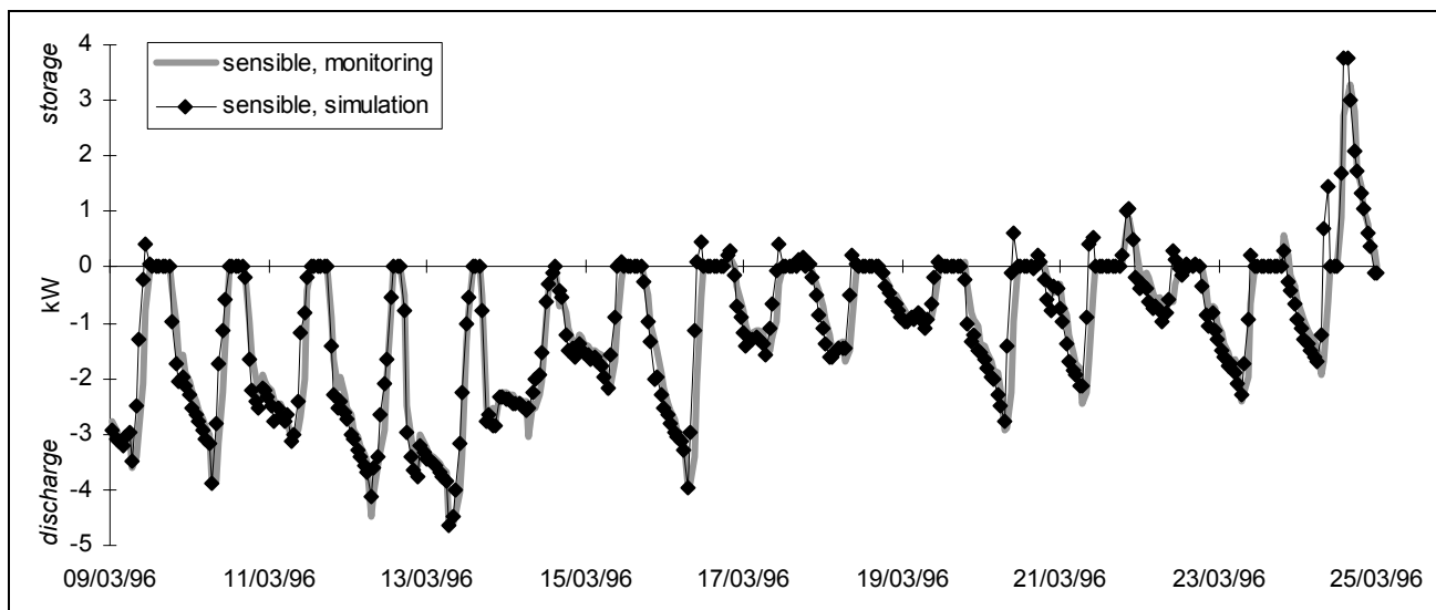
Fig. 6 : Hourly sensible heat exchange (from air to soil) for one of the two branches of the « Caroubier » earth channel : monitored and simulated over a winter month.
