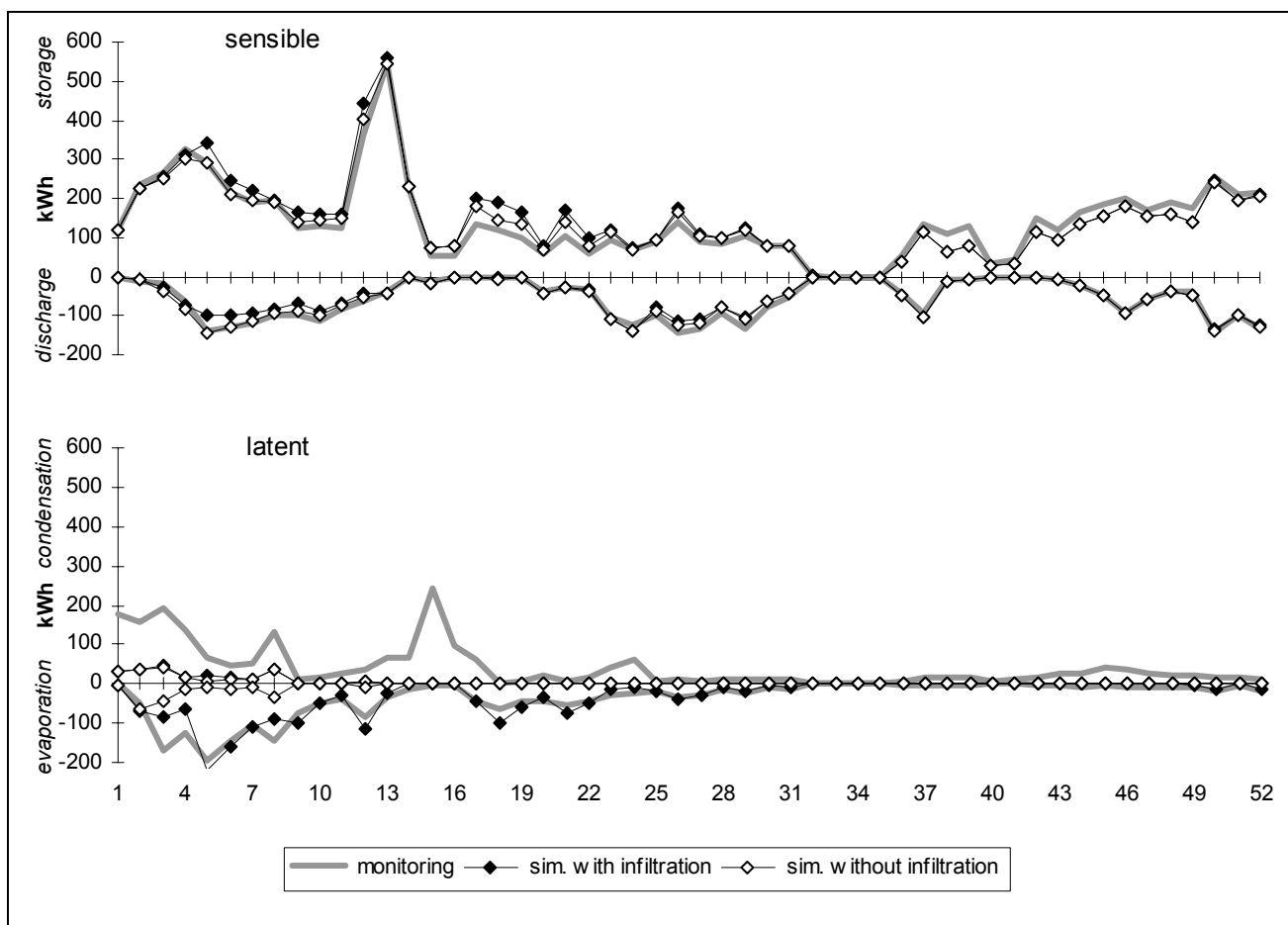
Fig. 4 : Weekly sensible and latent energy exchanges (from air to soil) for « Geoser » earth-channel over one year (April 94 – March 95).
