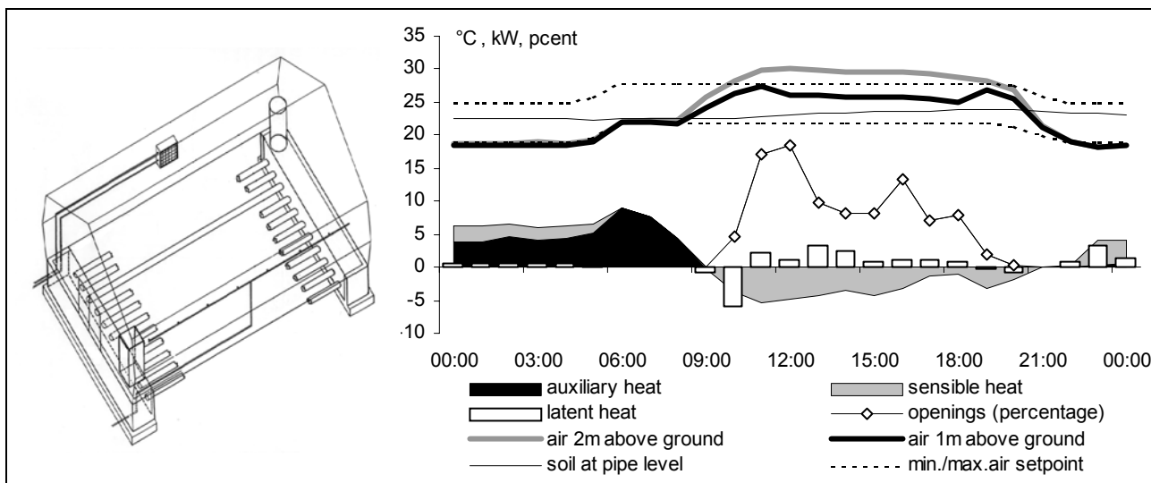
Fig. 1 : « Geoser » experiment of underground heat storage in agricultural greenhouses : schematic layout and operation on May 10 th , 1994.
