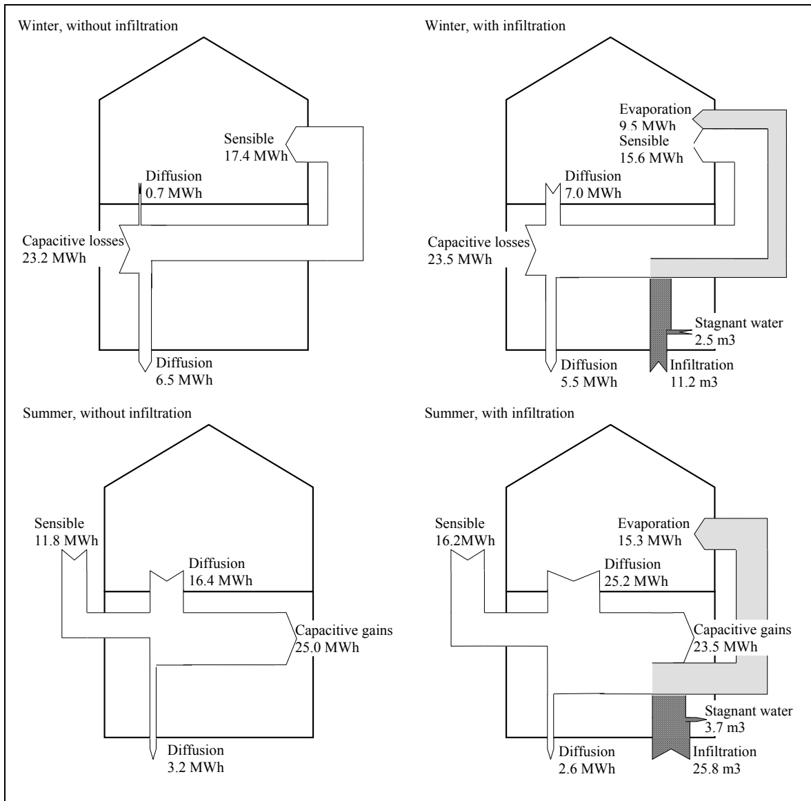
Fig. 8 : Seasonal simulated energy and water balance for « Schwerzenbacherhof » buried pipe system, with and without infiltration.
