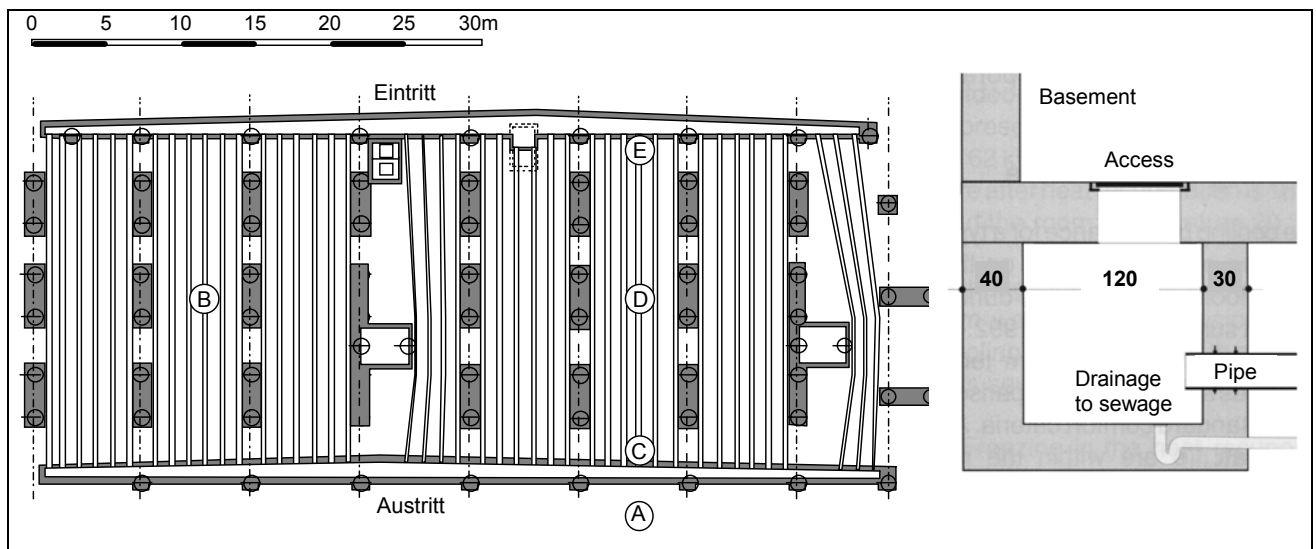
Fig. 7 : General layout and construction detail of « Schwerzenbacherhof » cooling and preheating system.
