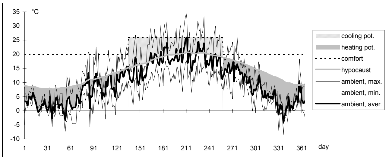
Fig. 9 : Ambient temperature profile for the city of Geneva, as well as cooling and heating potential of the « Caroubier » buried pipe system as constructed.
