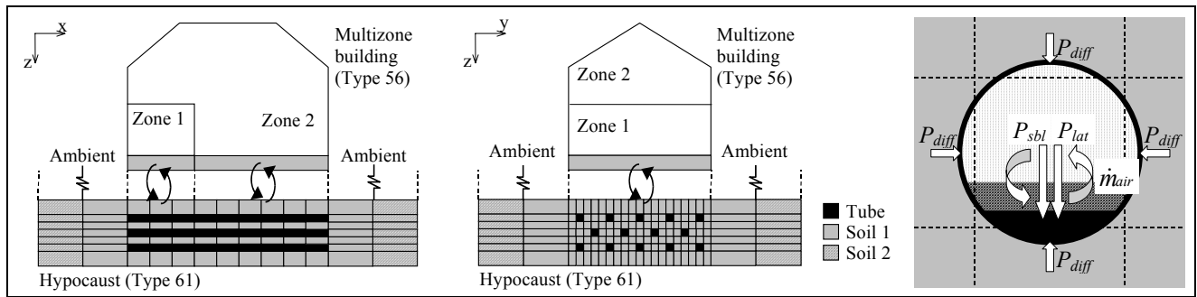
Fig. 2 : Example of earth channel geometry (various pipe layers, inhomogenous soils, different border conditions) and linking to other TRNSYS simulation models, as well as detail of energy/moisture exchange between air and tube.
