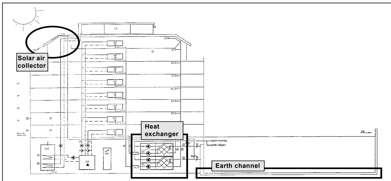
Fig. 5 : General layout of heating and fresh air preheating system for the « Caroubier » building.
