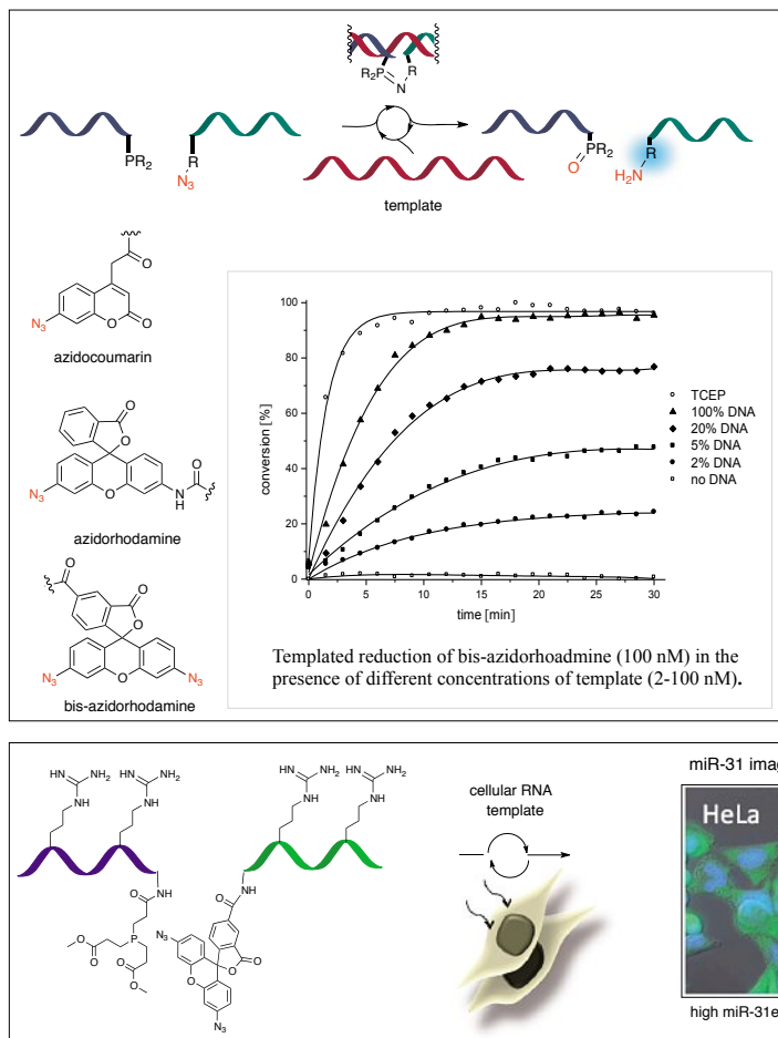
Fig. 9. Imaging of cellular nucleic acids using a templated Staudinger reduction with cell permeable GPNA.
