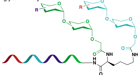
Fig. 2. A. Schematic representation of PNA-encoded synthesis (PES). B. Selected examples of library reported by our lab using PES.
