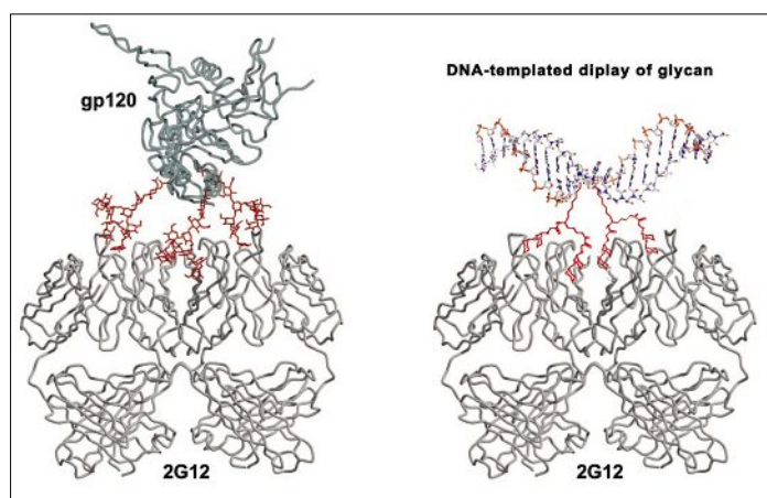
Fig. 4. Model of antibody 2G12 (left) binding HIV's oligosaccharide epitope (left, image adapted from D. A. Clarese, et al. , Science , 2003, 300, 2065) and schematic representation of templated assembly of a mannose disaccharide emulating HIV's epitope (right).
