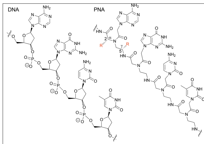
Fig. 1. DNA and PNA structures. Chemical structures of DNA (left) and PNA (right). Modifications at the \alpha or \gamma position of PNA (R) are tolerated and may even enhance DNA or RNA hybridization.
