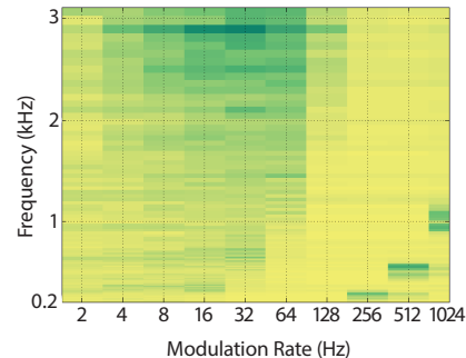
Fig. 3. Auditory temporal modulation feature matrix.
