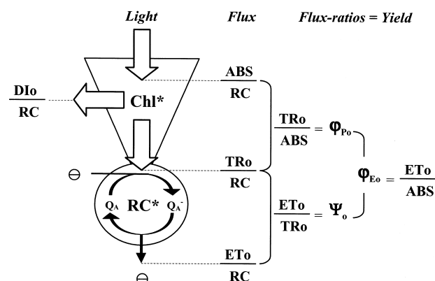
Figure 2. Energy cascade from solar light to photosynthetic electron transport in chloroplasts. ABS refers to the photon flux absorbed by the chlorophyll antenna pigments Chl^* of the photosystem II. Part of this excitation energy Dlo is dissipated, mainly as heat and less as fluorescence emission. Another part is channelled to the reaction centre RC, as trapping flux TRo . In the reaction centre, the excitation energy is converted into redox energy by reducing the electron acceptor Q_A to Q_A^- , which is then reoxidised to Q_A , creating an electron transport ETo . The three yields \Phi_{Po} , \Psi_o and \Phi_{Eo} are directly related to the three energetic fluctuations, as the ratio of any two of them. The maximum quantum yield of primary photochemistry \Phi_{Po} = TRo/ABS represents the probability that an absorbed photon is trapped by the RC and used for primary photochemistry, reducing Q_A to Q_A^- . \Psi_o = ETo/TRo represents the efficiency with which a trapped exciton moves an electron further than Q_A^- in the electron transport chain. \Phi_{Eo} ( = ETo/ABS ) represents the probability that an absorbed photon moves an electron into the electron transport chain. Therefore \Phi_{Eo} = \Phi_{Po} \cdot \Psi_o .
