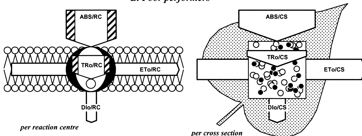
Figure 6. Energy pipeline models of the high performer (A) and poor performer (B) trees. The membrane models (left) represent the specific activities, expressed as fluctuation per reaction centre (RC). The leaf models (right) show the phenomenological fluctuations, expressed as per leaf cross section (CS). The relative magnitude of each activity or fluctuation is shown by the width of the corresponding arrow. The average antenna size is given as ABS/RC. This expresses the total absorption flux of PSII antenna chlorophyll divided by the number of active (in the sense of Q_A reducing) reaction centres. Thus, the antenna of PSII complexes with non- Q_A reducing RCs (so called heat sink centres) are graphically added to the antenna of the active reactions centres. The absorption and trapping by PSII units with a heatsink centre is indicated as the hatched parts of the arrows ABS/RC and TRo/RC. The antenna belonging to the PSII units with heat sink centres is drawn in black while the antenna which belongs to the active ( Q_A reducing) centres is drawn in white. In shaded zones of the leaf model, the Q_A reducing RCs per cross section are indicated by open circles and the non Q_A reducing RCs (heat sink or silent RCs) are indicated by the closed circles. The colouration of the foliage indicates the chlorophyll concentration per leaf cross section.
