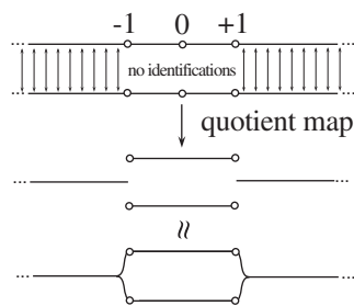
FIGURE 5. Another non-Hausdorff manifold
