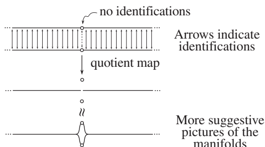
FIGURE 4. The line with two origins
