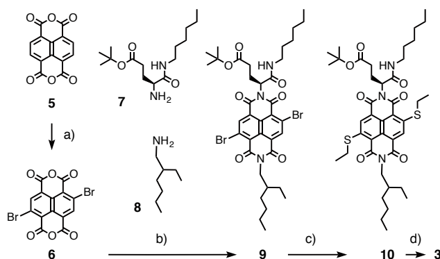
Scheme 1. Synthesis of catalyst 3 . a) Dibromoisocyanuric acid, \text{H}_2\text{SO}_4 , rt, 12 h, 76%, 4,28 b) AcOH, 80 °C, c) EtSH, 18-crown-6, \text{K}_2\text{CO}_3 , \text{CHCl}_3 , 75 °C, d) TFA, \text{CH}_2\text{Cl}_2 .
