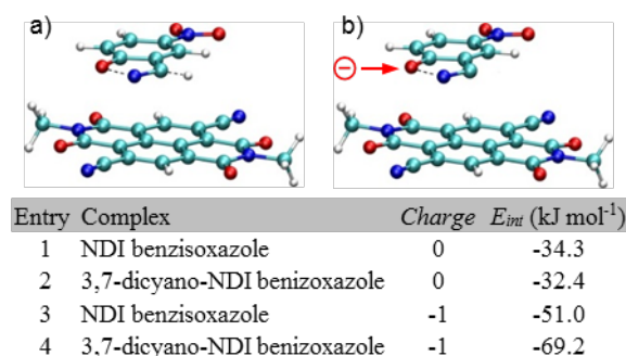
Figure 6. Model for transition state complexes of a) neutral and b) negatively charged complexes of benzisoxazole with N,N-dimethyl NDI. For both unsubstituted and dicyano-substituted substrates the BSSE corrected binding energies are computed with the IEFPCM/M06-2X/Def2-TZVP method.
