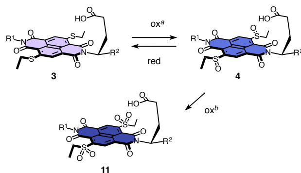
Figure 7. Structure of the catalysts 3 and 4 . R 1 and R 2 as in Figure 3. a MCPBA, CH 2 Cl 2 , 0 °C; b MCPBA, CH 2 Cl 2 , room temperature.
