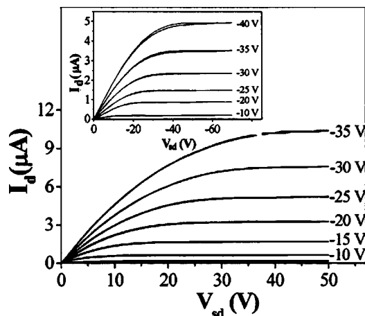
FIG. 2. Source-drain current vs source-drain voltage measured at different gate voltages for a device fabricated on \text{SiO}_2 , with an L=1.2 \text{ mm} channel length and W=200 \mu\text{m} channel width. The inset shows similar data for a FET fabricated using parylene C ( L=650 \mu\text{m} , W=340 \mu\text{m} ).
