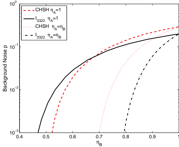
FIG. 2: Minimal detection efficiency \eta_B required for a given noise power. The curves for the symmetric case, \eta_A = \eta_B , are also plotted, the curve for CHSH being Eberhard's result. Though CHSH provides a larger threshold efficiency for any noise power than I_{3322} in the symmetric case, I_{3322} can tolerate smaller efficiencies than CHSH when p < 6\% and \eta_A = 1 . This is probably due to the fact that inequality I_{3322} is asymmetric, contrary to CHSH.
