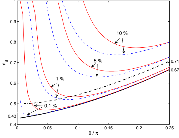
FIG. 1: (Color online) Numerical optimization of the threshold efficiency \eta_B^{th} as a function of \theta . Thick lines: pure states result for CHSH (dashed-dotted line) and I_{3322} (full line). Thin full lines: I_{3322} for states (6); thin dashed lines: I_{3322} for states (7); with error value for both.
