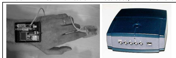
Fig. 3: Self supporting sensor and front-end, ECG sensors
