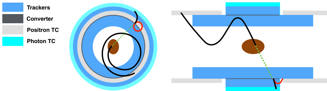
Fig. 6 Sketches of a detector design made of an extended e^+ and an e^+e^- pair trackers (sky blue) separated by a thin conversion layer (dark gray, not in scale), with positron (light gray) and photon (cyan) timing
