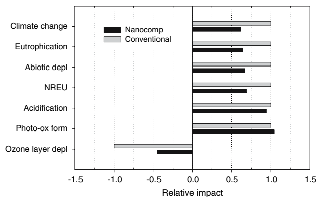
Fig. 3 Relative results of the impact assessment of agricultural film
