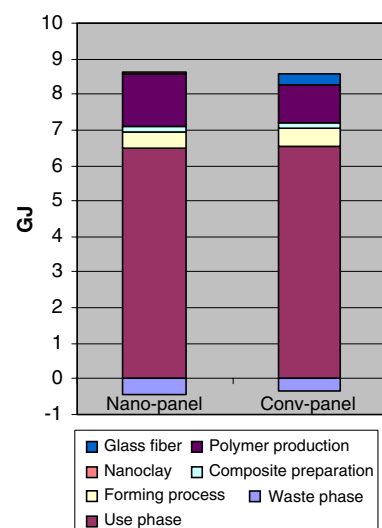
Fig. 5 NREU of one functional unit of automotive panels (cradle-to-grave)
