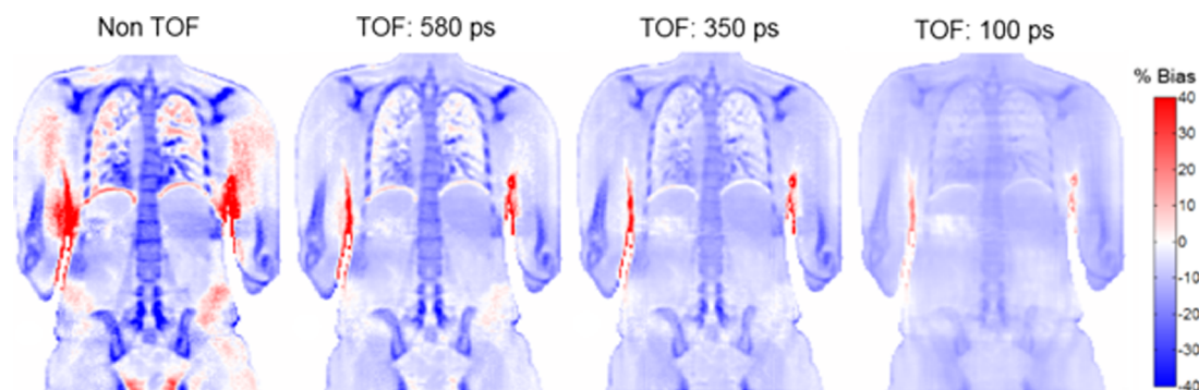
FIG. 7. Bias maps between PET image reconstructed by the four-class MRAC and CTAC maps without TOF and with different TOF resolutions in a whole-body phantom simulated from a clinical study. Adapted with permission from A. Mehranian and H. Zaidi, "Impact of time-of-flight PET on quantification errors in MRI-based attenuation correction," J. Nucl. Med. 56 (4), 635–641 (2015). Copyright 2015 by SNMMI.
