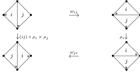
FIGURE 6. Inversion relation (3.9).
