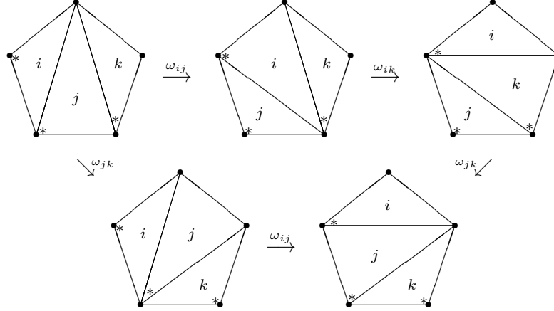
FIGURE 5. Pentagon relation (3.8).
