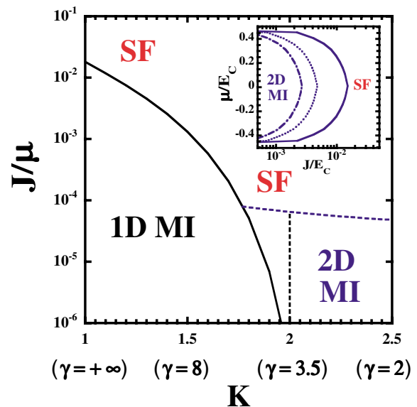
FIG. 1 (color online). Zero-temperature phase diagram of a 2D lattice of coupled 1D boson systems. The values on the vertical axis are defined up to a factor of order unity. K is the TLL parameter. The corresponding values of \gamma = Mg/\hbar^2\rho_0 are also given. A periodic potential of amplitude u_0 , commensurate with the density \rho_0 , is applied longitudinally ( u_0 \approx 0.03\mu for K = 1 and u_0 \approx 0.02\mu for K = 2.5 ). For infinite 1D systems only two phases exist: a 1D Mott insulator (1D MI) and a 3D (but anisotropic) superfluid (SF). For finite tubes, a 2D Mott insulator (2D MI) can exist for J/\mu below the horizontal dashed curve (we have taken N_0 = 100 atoms per 1D tube). The vertical dashed line (schematic) indicates that the transition to the 1D MI should take place for K \approx 2 . The inset is the phase diagram of a 2D optical lattice of finite 1D systems for u_0 = 0 and N_0 = 100 , as a function of chemical potential \mu and the hopping J , and for K = 1 (continuous curve), K = 2 (dotted curve), K = 4 ( \gamma = 0.71 , dash-dotted curve).
