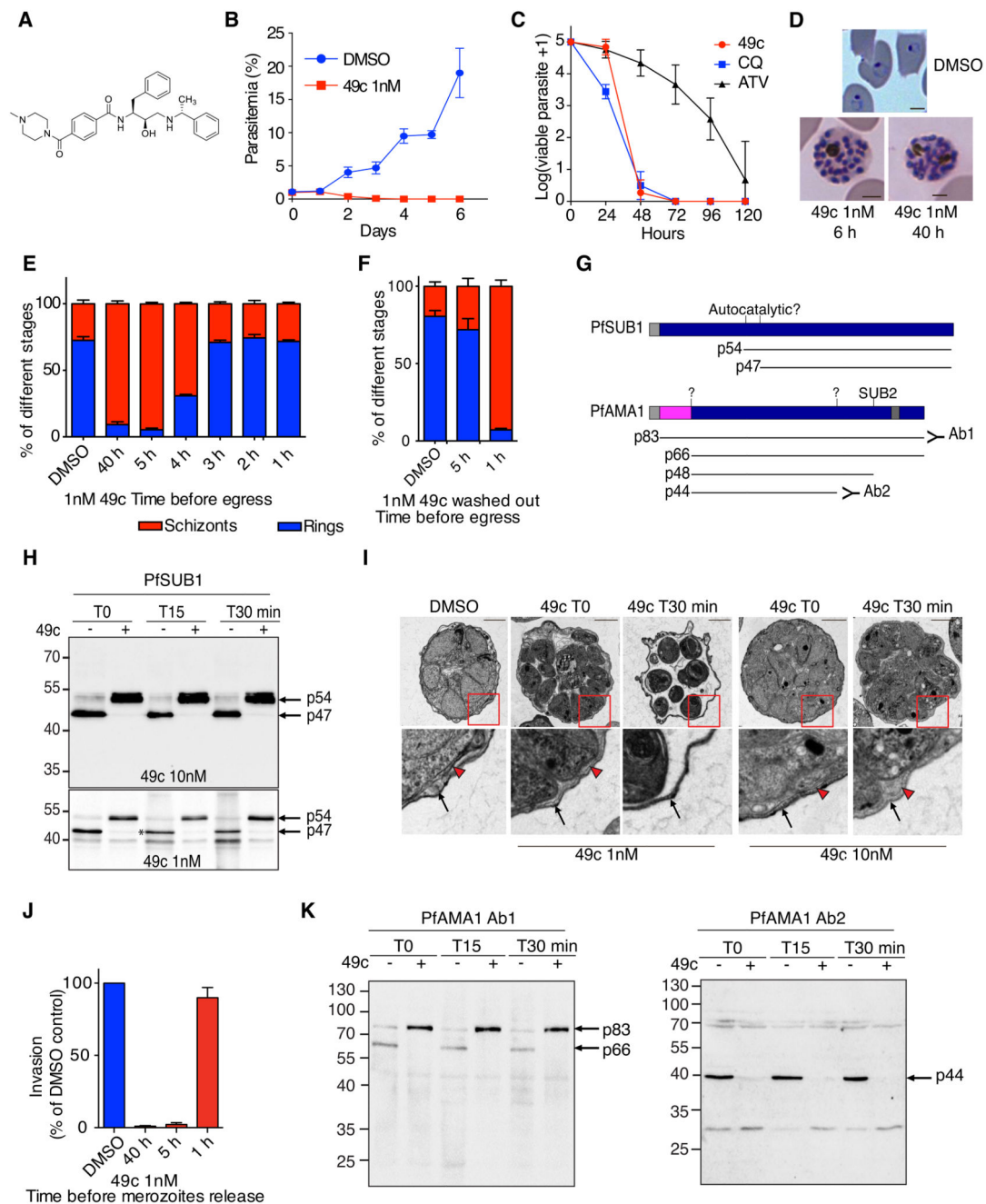
Figure 1. Compound 49c prevents Plasmodium falciparum merozoite egress and invasion.
