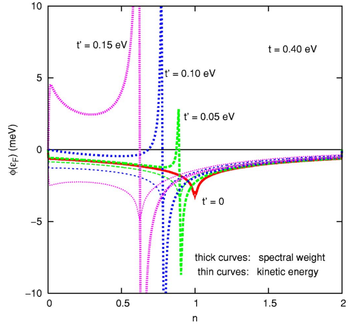
FIG. 5. (Color online) The finite-temperature correction to the optical spectral weight (thick curves), for various values of t' , as indicated. Also plotted is the analogous quantity for the kinetic energy [which, by Eq. (8), is just -8tg(\epsilon_F) ]. Note that the latter is always negative, while the spectral weight becomes positive for a finite electron concentration for electron (hole) densities below (above) the van Hove singularity. The magnitude of the anomalous region increases with increasing t' .
