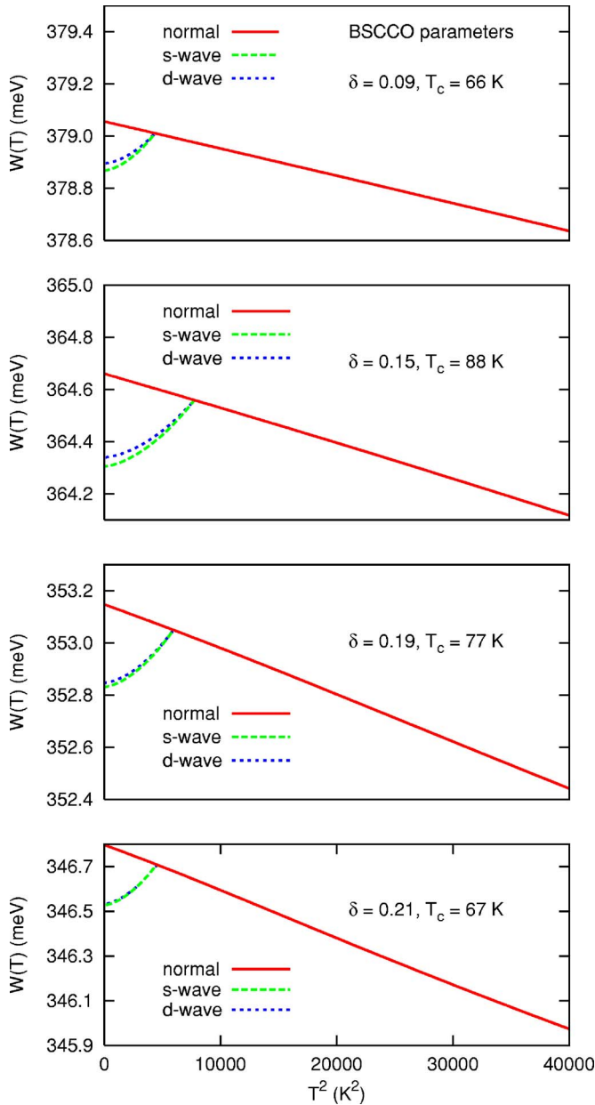
FIG. 7. (Color online) Spectral weight for the four hole doping concentrations (along with their measured T_c 's) considered in the experiments (Ref. 14). These calculations use the ARPES-determined band structure parameters from Ref. 24, including the bilayer splitting. Slopes are always negative, and the change at T_c is also always negative. Note that in this case the s -wave order parameter gives roughly the same value as the d -wave parameter.
