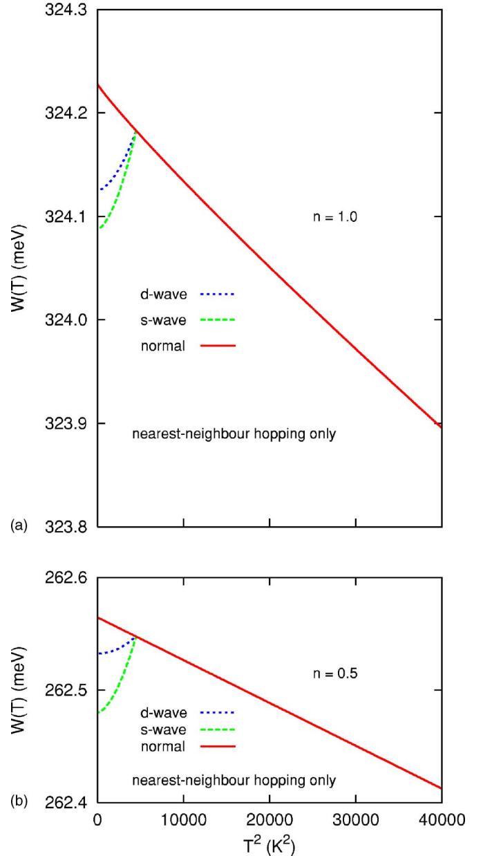
FIG. 1. (Color online) Spectral weight vs T^2 for (a) half-filling and (b) n=0.5 . The normal state is given by the solid red curve, and the superconducting state with d -wave ( s -wave) symmetry by the short-dashed blue (dashed green) curve. In both cases the normal-state result is almost linear in T^2 and the superconducting state shows a decrease in the spectral weight (increase in the kinetic energy) as expected. We used t=0.4 eV and BCS values for order parameters, etc., with T_c=69 K.
