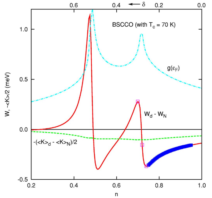
FIG. 8. (Color online) Spectral weight difference (solid red curve) as a function of electron concentration for the band structure determined by ARPES (Ref. 24). For simplicity we put T_c=70 K for all electron densities. The normal-state slope shows very similar behavior. Also plotted is the negative of the change in the kinetic energy (dashed green curve) and the density of states at the Fermi level (dot-dashed cyan curve), for reference. Note that “anomalies” in the spectral weight occur at the two van Hove singularities, while the change in kinetic energy is simply gently modulated by the density of states. Also shown with solid blue symbols is the hole doping regime of relevance to the BSCCO experiments in Ref. 14 and considered in the previous figure. For clarity only d -wave results are shown. The three open squares show the doping concentrations considered in the next figure, of possible relevance for overdoped samples with chemical potential that crosses the van Hove singularity (Ref. 30).
