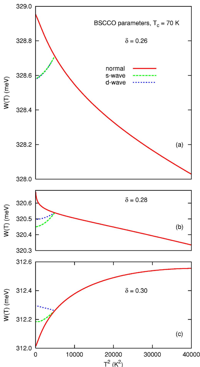
FIG. 9. (Color online) Spectral weight for three hole doping concentrations that move the chemical potential across the first van Hove singularity (see Fig. 8). Note the dramatic change that occurs as one dopes across the van Hove singularity (see text).
