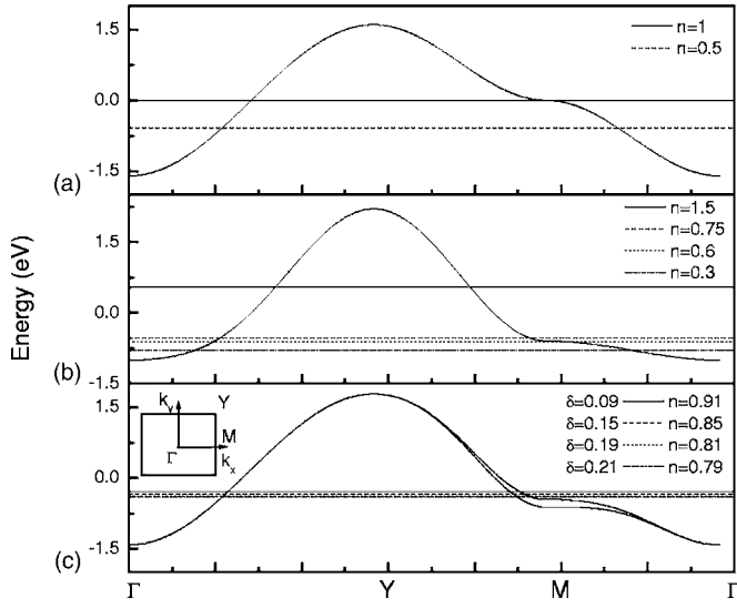
FIG. 3. Illustrative plots of the band structure for (a) nearest-neighbor hopping only, (b) the t - t' model, and (c) parametrization of Kordyuk et al. (Ref. 24) of the band structure with bilayer splitting. The van Hove singularities occur where the band dispersion flattens.
