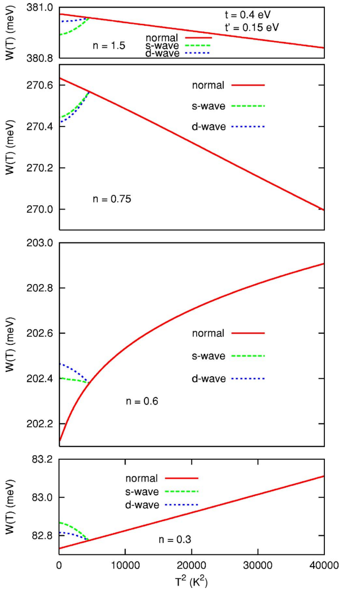
FIG. 6. (Color online) Spectral weight for four representative densities for the t - t' model (see Fig. 5). The progression from top to bottom is from high electron concentration to low electron concentration. Note the qualitative change from negative slope (lower-superconducting vs normal-state difference) to positive slope (higher-superconducting vs normal-state difference) as the electron concentration changes such that the chemical potential sweeps through the van Hove singularity.
