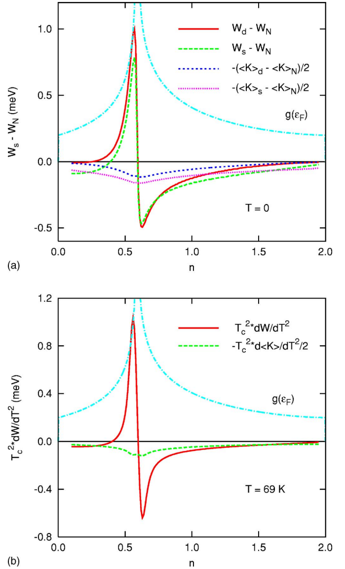
FIG. 4. (Color online) (a) The difference (W_d - W_N) in the spectral weight between the superconducting state with d -wave symmetry and the normal state at zero temperature vs doping (solid red curve), for the t - t' band structure, with t=0.4 eV and t'=0.09 eV. The dashed green curve shows the same quantity for s -wave symmetry. Both exhibit positive values to the left of the van Hove singularity (the density of states at the Fermi level is indicated, as a function of doping, by the dot-dashed cyan curve). The negative of the kinetic energy for d -wave (blue short-dashed curve) and for s -wave (dotted pink curve) symmetry behaves as expected, always negative, and peaks (in absolute value) at the van Hove singularity. (b) The normal-state slope (taken at T_c=69 K) of the spectral weight vs doping (solid red curve). The dashed green curve shows the same quantity for the negative of the kinetic energy. These behave in very similar fashion to the differences (taken at zero temperature) shown in (a).
