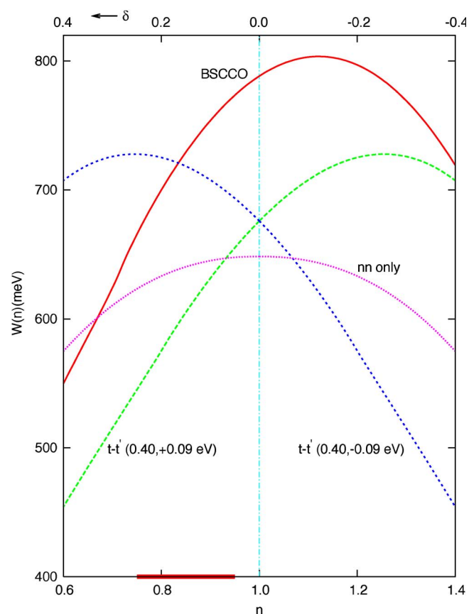
FIG. 10. (Color online) Spectral weight at zero temperature in the normal state vs electron concentration for four different band structures: that applicable to BSCCO (solid red curve), the t - t' model with t=0.40 eV and t'=0.09 eV (long-dashed green curve) and with t'=-0.09 eV (short-dashed blue curve), and the nearest-neighbor hopping only model, with t=0.40 eV. The three models that are physically relevant to the hole-doped cuprates (LSCO and BSCCO) have non-negative next nearest-neighbor hopping ( t' ) and show a spectral weight that decreases with increasing hole doping \delta over the relevant hole doping regime (see thick solid red line along the bottom axis). See text for further discussion.
