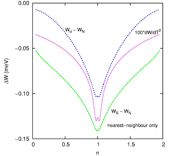
FIG. 2. (Color online) The difference ( W_d - W_N ) in the spectral weight between the superconducting state with d -wave symmetry and the normal state at zero temperature vs doping (dotted blue curve). The dashed green curve shows the same quantity for s -wave symmetry, and the pink points indicate the slope (with respect to T^2 ) of the spectral weight near T_c . All three quantities are always negative and show an enhancement near half-filling due to the van Hove singularity. In fact, the pink points are almost a perfect inverted image of the density of states [see the minus sign in Eq. (8)], except for the small density regime near half-filling, where the van Hove singularity makes the Sommerfeld expansion invalid.
