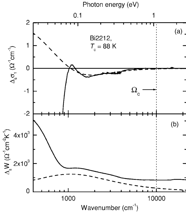
FIG. 5. (a) Slope-difference conductivity \Delta_s \sigma_1(\omega) of optimally doped Bi2212. (b) The corresponding integrated spectral weight \Delta_s W(\omega) . The dashed lines show a model which mimics the narrowing of the Drude peak.
