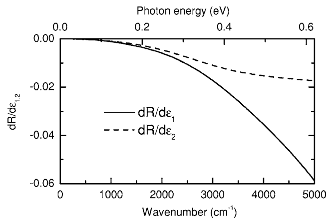
FIG. 6. The “sensitivity functions” (\partial R/\partial\epsilon_1)(\omega) and (\partial R/\partial\epsilon_2)(\omega) in the near and far infrared, obtained for Bi2212 near optimal doping at T_c=88 K as described in Appendix B.
