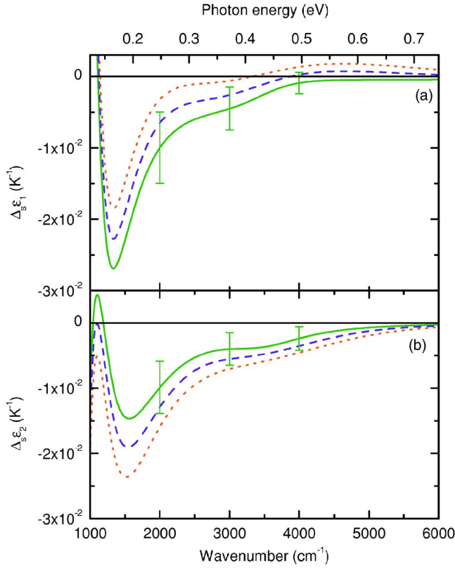
FIG. 4. (Color online) The continuation of the model slope-difference curves \Delta_s\epsilon_1(\omega) (a) and \Delta_s\epsilon_2(\omega) (b) of Fig. 3(b) to the midinfrared region, where only the reflectivity was measured. The colors and types of curves correspond to the ones in Fig. 3 (namely, the solid green curve is the best fit of all data, without any assumptions about the integrated spectral weight, while the dashed blue and dotted red curves are the fits with artificial constraints on the spectral weight). Note that the error bars, which are estimated as described in the text, are significantly increasing as the frequency is lowered.
