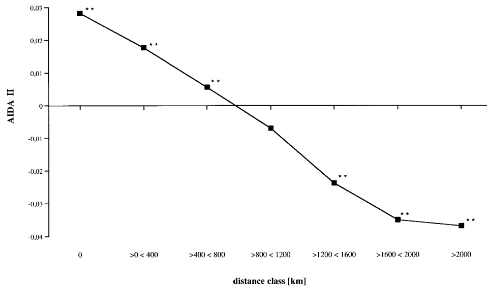
Figure 4 Correlogram of the AIDA II for 189 mtDNA haplotypes (HV1 sequences plus the Hpa I restriction site) from the Nile River Valley. The value of II is the Y-axis, whereas the X-axis is the width of arbitrarily chosen distance classes. The double asterisks (**) denote that the value of II for all distance classes except 800–1,200 km differs significantly ( P < .01 ) from 0.
