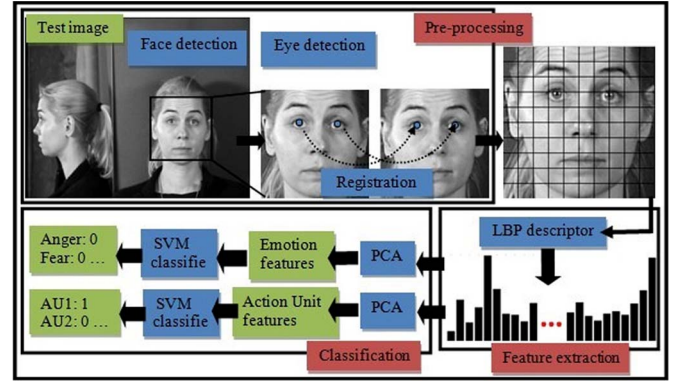
Fig. 2. Overview of the FERA 2011 baseline system for detection of 12 AUs and 5 emotions.
