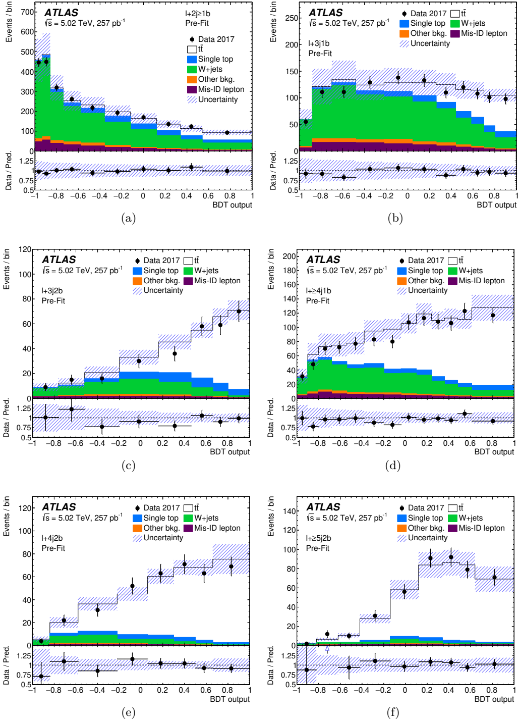
Figure 5. Comparison of the data and predicted BDT output distributions for the (a) \ell + 2j \geq 1b region, (b) \ell + 3j \text{ } 1b region, (c) \ell + 3j \text{ } 2b region, (d) \ell + \geq 4j \text{ } 1b region, (e) \ell + 4j \text{ } 2b region, and (f) \ell + \geq 5j \text{ } 2b region. The pre-fit uncertainties are shown. The ‘Other bkg.’ includes Z + jets and diboson backgrounds. The blue hashed lines correspond to the total uncertainty of the prediction in a given bin. The lower panels show the ratio of the data to the prediction, along with the uncertainty in the ratio.
