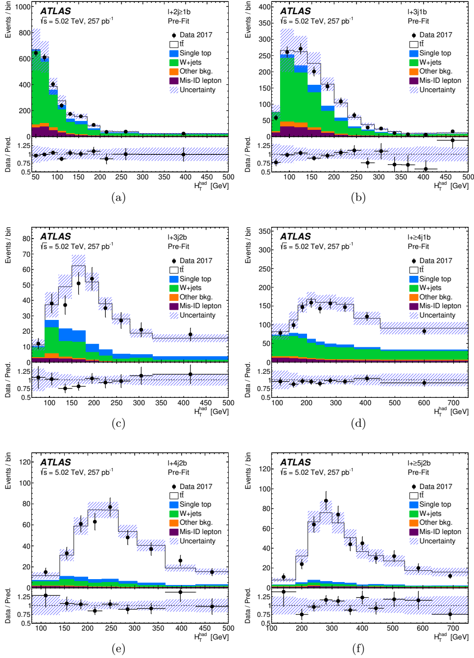
Figure 4. The observed and predicted distributions of H_T^{\text{had}} in the (a) \ell + 2j \geq 1b region, (b) \ell + 3j \text{ } 1b region, (c) \ell + 3j \text{ } 2b region, (d) \ell + \geq 4j \text{ } 1b region, (e) \ell + 4j \text{ } 2b region, and (f) \ell + \geq 5j \text{ } 2b region. The pre-fit uncertainties are shown and the last bin contains the overflow. The ‘Other bkg.’ includes Z + jets and diboson backgrounds. The blue hashed lines correspond to the total uncertainty of the prediction in a given bin. The lower panels show the ratio of the data to the prediction, along with the uncertainty in the ratio.
