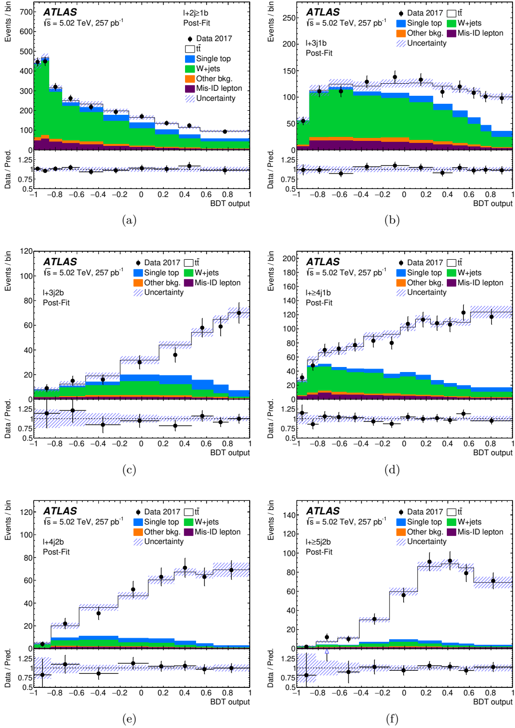
Figure 7. Comparison between data and the results of the fit to the BDT output distributions in the (a) l+2j \geq 1b region, (b) l+3j \text{ } 1b region, (c) l+3j \text{ } 2b region, (d) l+\geq 4j \text{ } 1b region, (e) l+4j \text{ } 2b region, and (f) l+\geq 5j \text{ } 2b region. The ‘Other bkg.’ includes Z + jets and diboson backgrounds. The bottom panel displays the ratio of data to the total prediction. The hashed area represents the total uncertainty of the background.
