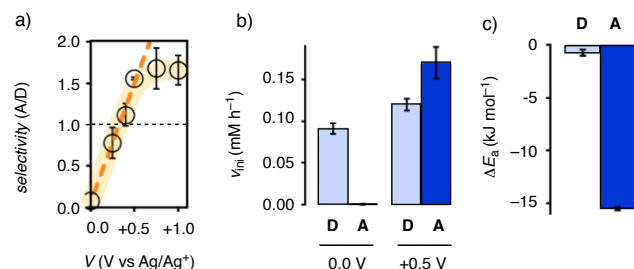
Figure 4. a) Dependence of A/D product ratio on the potential applied to catalyst 1 . Shown are average values from at least two independent experiments \pm error, with linear curve fit for the first four data points. The open circuit potential was 0.040 \pm 0.025 \text{ V} . b) Initial velocity of the formation of product D and A in the presence of catalyst 1 at 0.0 V (cyan) and +0.5 V. c) Transition-state stabilization by +0.5 V for decarboxylation D and addition A on catalyst 1 , calculated from changes in v_{\text{ini}} in (b).
