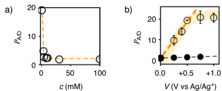
Figure 5. a) Dependence of P_{A/D} with catalyst 1 at V = +0.5 V on the concentration c of TBA nitrate. The ionic strength was maintained by reducing the concentration of TBAPF 6 (100 - c mM). b) Dependence of P_{A/D} on the potential applied to catalyst 1 in the absence (○) and the presence (●) of 4.0 mM nitrate, with linear curve fit for the first four data points.
