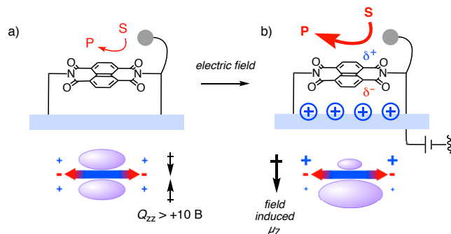
Figure 1. The concept of electric-field-assisted anion- \pi catalysis. (a) Bifunctional anion- \pi catalysts composed of, e.g., a \pi -acidic NDI with Q_{zz} > +10 B and an amine base (grey circle) are immobilized on conducting surfaces (light blue). (b) Application of an electric field induces macrodipole \mu_z , which in turn increases the stabilization of anionic intermediates and transition states between substrate S and product P on the polarized \pi surface of the catalyst.
