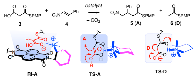
Figure 3. With MAHT 3 , enolate addition to yield product A and decarboxylation to product D are in kinetic competition. Discrimination between planar ( RI-A , TS-A ) and twisted ( TS-D ) tautomers on \pi -acidic surfaces with tightly ( RI-A , TS-A ) but not loosely ( TS-D ) interfaced base catalysts can provide selective access to the disfavored but relevant A .
