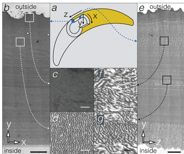
Fig. 2 (a) Schematic representation of the 3D coordinates of the egg sac. (b–e) TEM micrographs of egg sac cross sections in the XY (b–d) and YZ (e–g) planes. Scale bars: 10 \mu\text{m} (b and e), and 0.5 \mu\text{m} (c, d, f and g).
