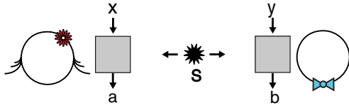
FIG. 1 (color online). Sketch of a Bell experiment. A source ( S ) distributes two physical systems to distant observers, Alice and Bob. Upon receiving their systems, each observer performs a measurement on it. The measurement chosen by Alice is labeled x and its outcome a . Similarly, Bob chooses measurement y and gets outcome b . The experiment is characterized by the joint probability distribution p(ab|xy) of obtaining outcomes a and b when Alice and Bob choose measurements x and y .
