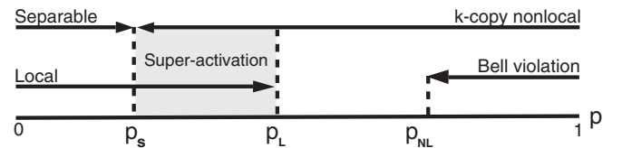
FIG. 6. Nonlocal properties of the isotropic state (53). The state is separable for p \leq p_s = 1/(d+1) , admits a local model for p \leq p_L ( Almeida et al. , 2007 ), and violates a Bell inequality for p_L < p_{NL} < p ( Collins, Gisin, Linden et al. , 2002 ). In the interval p_L < p < p_{NL} , it is not known whether the state admits a local model or, on the contrary, violates a Bell inequality. Finally, when several copies of the isotropic state can be measured jointly, nonlocality is obtained whenever a single copy of the state is entangled, that is, if p > p_s ( D. Cavalcanti et al. , 2013 ). In the gray region, superactivation of quantum nonlocality occurs ( Palazuelos, 2012a ).
