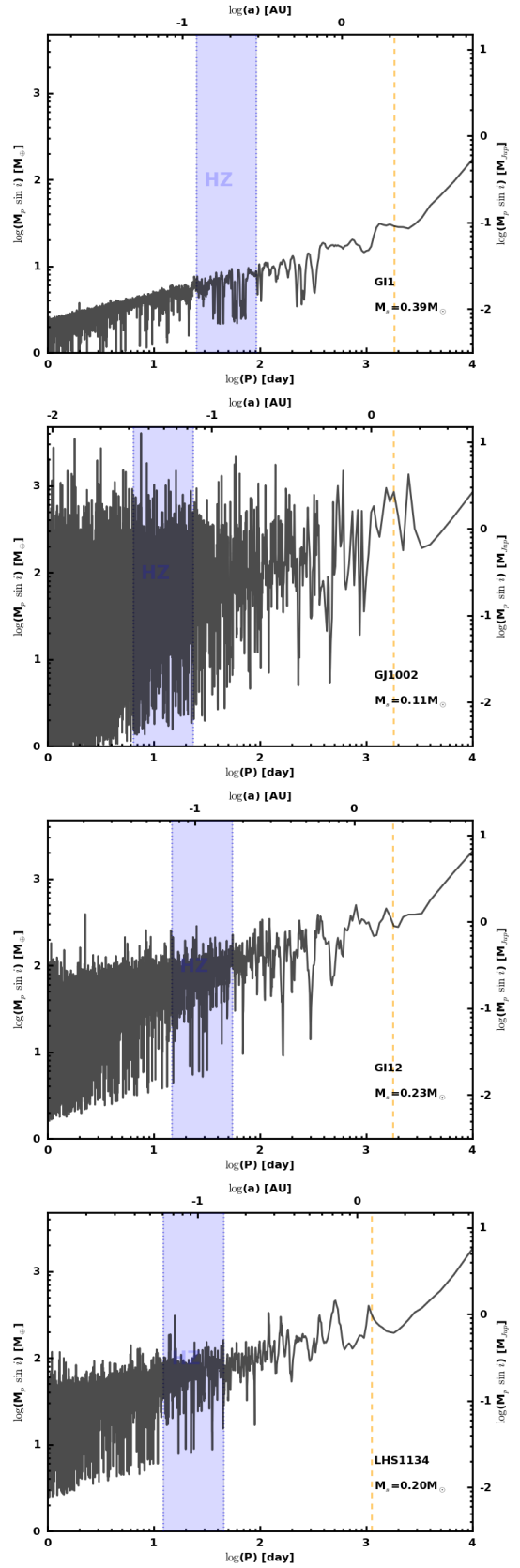
Fig. 19. Phase-averaged detection limits on m \sin i for time-series with more than four measurements. Planets above the limit are statistically excluded, with a 99% confidence level, for half the 12 trial phases. Some panels display two curves: the upper one is the detection limits before any model is subtracted and the bottom one is for the residuals around a chosen model (composed of planets, linear drifts, and/or a simple sine function). See Sect. 6 for details.
