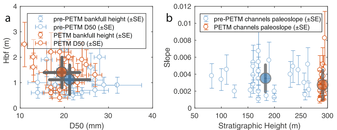
Figure 3. Channel deposits characteristics before and during the PETM global warming. (a) D50 and bankfull channel depth Hbf ( \pm SE) at pre-PETM (N = 26) and PETM (N = 22) field stations. Large circles indicate population mean ( \pm 1\sigma ). (b) Calculated palaeoslopes at individual field stations indicated with standard error. Larger circles indicate formation average palaeoslope ( \pm 1\sigma ).
