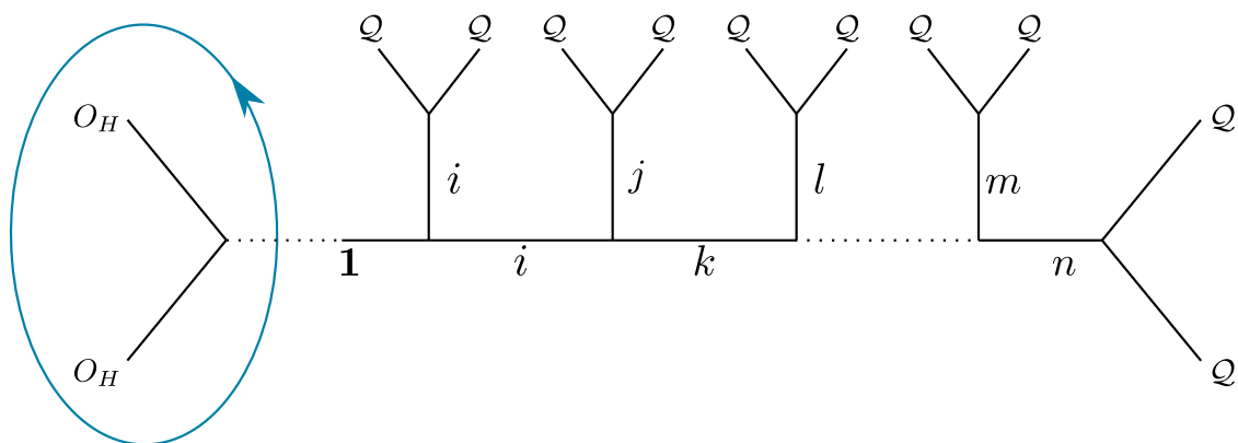
Figure 2: We will treat the Q operators as parametrically lighter than the O_H . We can then impose that the O_H fuse to the identity operator, which, to leading order results in \tilde{T}_{cl}(w \rightarrow \infty) = O(w^{-4}) .
