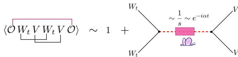
Figure 1: Application of our main result (4) to the butterfly effect (‘scrambling’) in heavy states, i.e. an out-of-time-order “HLLLL” correlation function. As indicated in purple, the effect of the heavy insertions can be interpreted as dressing the propagator, s^{-1} , of the leading mode, the “scramblon” [26], exchanged between the light operators on the second sheet by the exponential factor s^{-1} = e^{-i\alpha t} . In the ergodic phase, \alpha = i|\alpha| , this leads to maximal scrambling, while in the non-ergodic phase, \alpha = |\alpha| , this results in an oscillatory OTOC. The bulk interpretation of the scramblon picture is a single graviton exchange in the heavy background. Full details of the calculation summarized here can be found in section 4 below.
