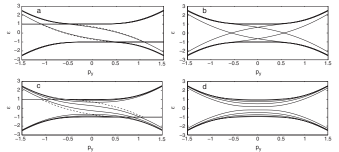
FIG. 3. Energy level structure in the presence of nonuniform interlayer bias \varphi(x) . The low-energy states in (a) and (c) are localized on the single kink of profile \varphi(x) = \tanh(x/\ell) with \ell = 0.5 and \ell = 4 , respectively. For (a) and (c) we used open boundary conditions, \Psi(\pm 20) = 0 , which caused flat bands at \varepsilon = \pm 1 . The dashed lines are the analytical expressions for the intragap state dispersion, Eq. (14). (b) Same as (a) but with kink and antikink at x = \pm 10 and periodic boundary conditions. (d) Nontopological confinement for potential profile \varphi(x) = \tanh^2(x/4) . Note the absence of chiral zero modes.
