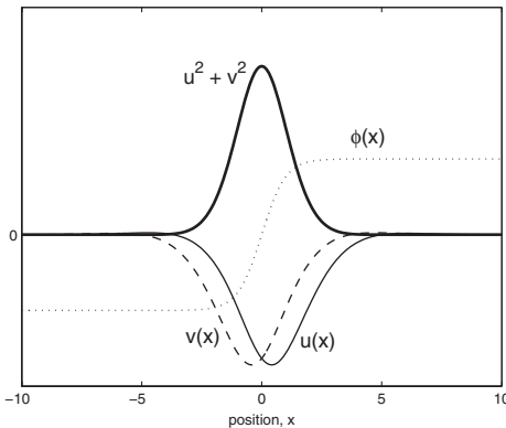
FIG. 2. Spatial structure of the confined state obtained numerically from Eqs. (5) and (6) for particular value p_y = -1/2^{3/4} . The energy of the state is \varepsilon = 0.1140 . Shown are the components u and v of the wave function (thin and dashed lines, respectively), the probability density |\Psi|^2 = u^2 + v^2 (thick line), and the potential profile, taken here as \varphi(x) = \tanh(x) . Note the symmetry, u(x) = v(-x) .
