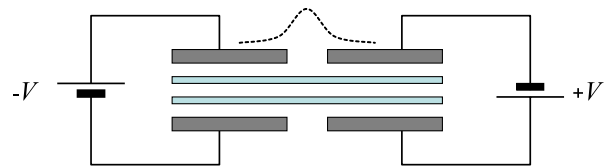
FIG. 1 (color online). Side view of a gated bilayer graphene configuration with the voltage kink. The region where the interlayer voltage changes sign (channel) supports bands of chiral zero modes (dashed line). The conventional (nontopological) confinement would correspond to the same polarity of bias on both sides of the channel.
