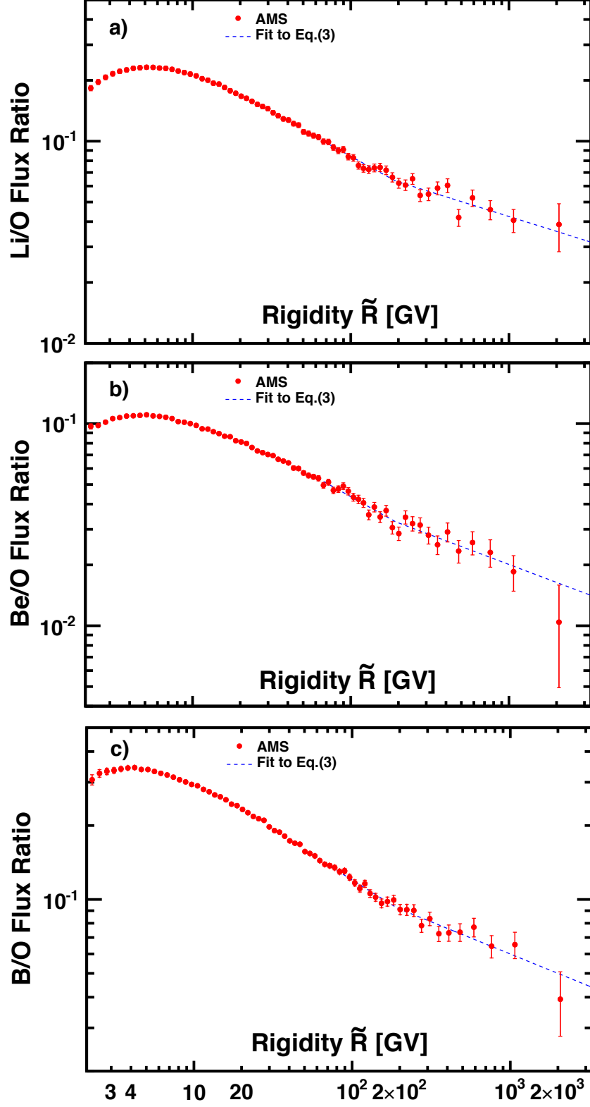
FIG. SM 10. The AMS (a) Li/O, (b) Be/O, and (c) B/O flux ratios as functions of rigidity together with the Eq. (3) fits (dashed lines) for the two rigidity intervals [192\text{--}3300] and [60.3\text{--}192] GV. The difference between the spectral indices in these rigidity intervals is 0.19 \pm 0.06 for Li/O, 0.15 \pm 0.07 for Be/O, and 0.14 \pm 0.05 for B/O.
