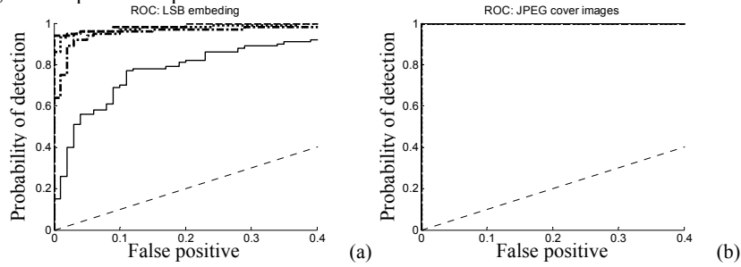
Fig. 7. ROCs for LSB embedding in raw images (a) and \pm 1 embedding in previously compressed JPEG images (b) with different capacity: solid = 0.25 bpp, dash-dotted = 0.5 bpp, dotted = 0.75 bpp, dashed = 1 bpp.
