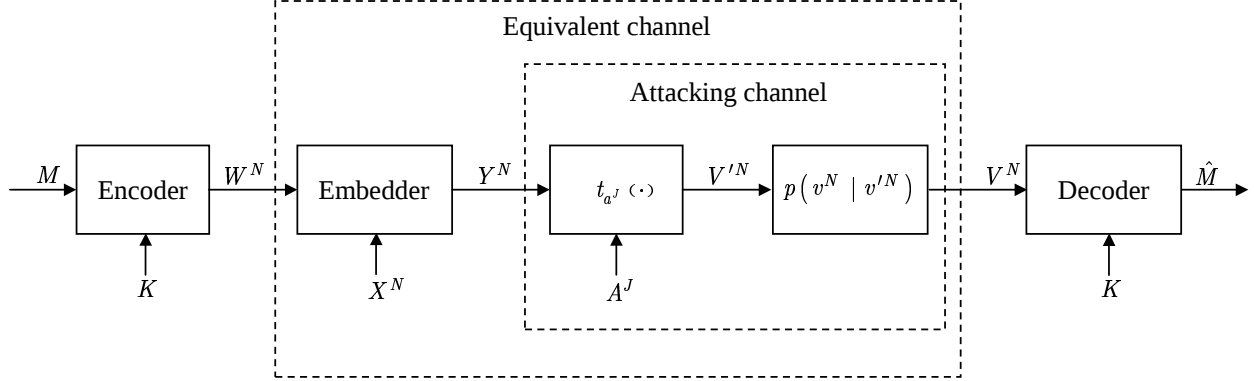
Figure 1. Considered communications setup.
