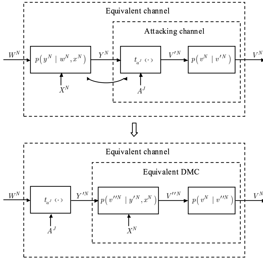
Figure 3. Possible structures of the equivalent channel.
