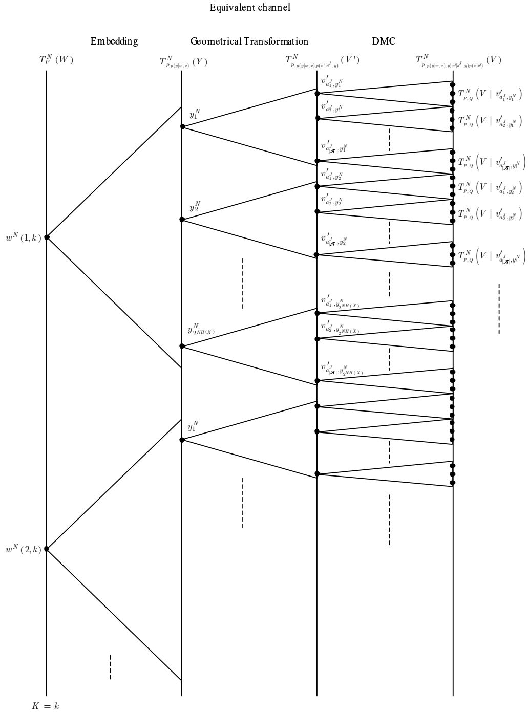
Figure 2. Codewords selection considering the equivalent channel.
