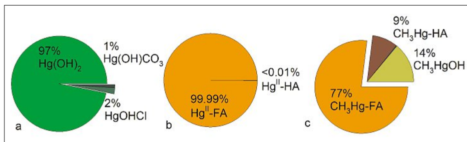
Fig. 2. Distribution of Hg species in a model lake water contaminated with Hg and containing 0.35 mg/L [\text{NO}_3^-] , 9.14 mg/L [\text{Cl}^-] , 43.64 mg/L [\text{SO}_4^{2-}] , 6.2 mg/L [\text{Na}^+] , 1.59 mg/L [\text{K}^+] , 40.7 mg/L [\text{Ca}^{2+}] , 5.9 mg/L [\text{Mg}^{2+}] at pH 8.3 and a dissolved organic matter concentration of 0.25 mg/L humic and 2.25 mg/L fulvic acids. The water composition corresponds to that measured in G3 sampling point of Lake Geneva in October 2013. Speciation was computed with the WHAM/Model VII chemical equilibrium program with updated formation constants for \text{OH}^- , \text{Cl}^- , \text{NH}_4^+ , \text{PO}_4^{3-} and \text{CO}_3^{2-} . [9] (a) 3.1 \times 10^{-10} M [\text{Hg}^{\text{II}}] , only inorganic complexes are considered; (b) 3.1 \times 10^{-10} M [\text{Hg}^{\text{II}}] , DOM is taken into account; (c) 3.1 \times 10^{-12} M [\text{CH}_3\text{Hg}] , DOM is taken into account. The complexes formed with fulvic and humic acids are the prevailing forms of \text{Hg}^{\text{II}} and \text{CH}_3\text{Hg} , as well as chloride and hydroxide complexes. Estimated free mercury concentration \text{Hg}^{2+} < 10^{-30} M and free methylmercury concentration \text{CH}_3\text{Hg}^{2+} < 10^{-15} M.
