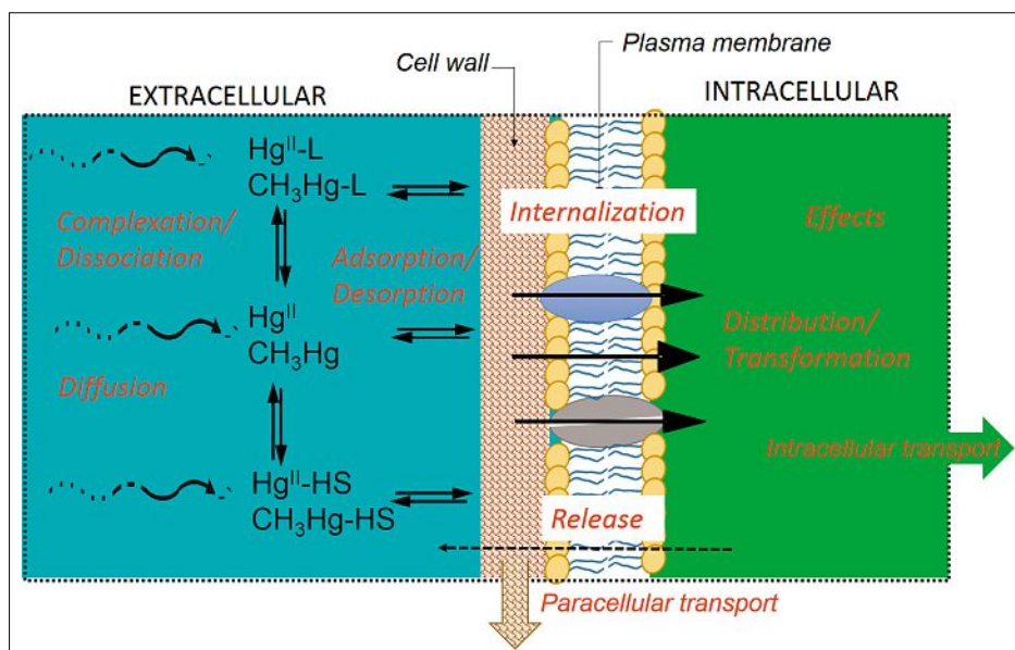
Fig. 3. Key processes determining the interactions of inorganic ( \text{Hg}^{\text{II}} ) and methylated Hg ( \text{CH}_3\text{Hg} ) forms with primary producers. Charges are omitted for simplicity.
