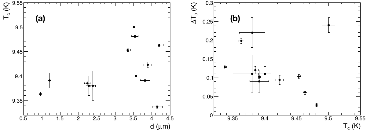
Figure 3. (a) Dependence of the critical temperature ( T_c ) values on the film thickness ( d ) for niobium films on copper analyzed in this study. (b) Dependence of the transition width ( \Delta T_c ) on the critical temperature.
