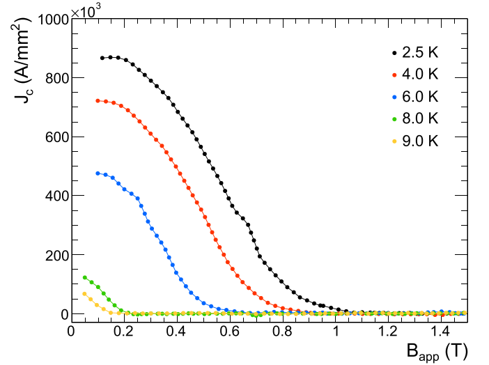
Figure 2. Critical current density ( J_c ) values of sample R11-C2 as a function of the applied magnetic field ( B_{\text{app}} ) at various temperatures.
