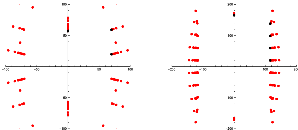
Figure 2: The Borel singularities for the free energies at large radius, for z = -15 \cdot 10^{-6} (left) and z = -10^{-8} (right). We use the poles of the Padé approximant and the free energies \mathcal{F}_g with g up to 120. The black dots in the first quadrant correspond to the tower \mathcal{A}_{0,n}^+ (194), for the values n = 0, 1 (left) and n = 0, 1, 2, 3 (right). The black dots in the positive imaginary axis corresponds to the location of the singularity (186) with \ell = 1 .
