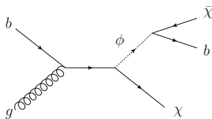
Fig. 2 Example of DM production in the b -FDM model
