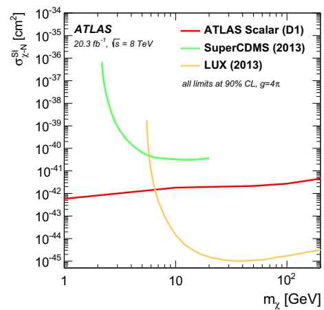
Fig. 5 Upper limits at 90 % CL on the spin-independent \chi -nucleon cross-section ( \sigma_{\chi-N}^{\text{SI}} ) for the scalar operator D1 (red) as a function of m_\chi . The yellow and green curves represent the exclusion limits recently set by the LUX and Super-CDMS collaborations [6, 7, 65]. The coupling is assumed to be g_q g_\chi = g = 4\pi
