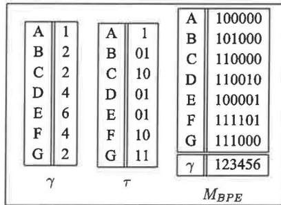
(a) Encoding of fig. 1.
