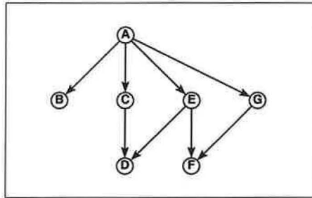
Figure 1 A small type hierarchy.
