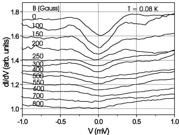
FIG. 4. Tunneling conductance as a function of bias, measured for different values of the applied magnetic field (the magnetic field is applied perpendicular to the \text{RuO}_2 planes; curves are offset for clarity). The data show that the low-bias suppression of the conductance disappears above the critical field.
