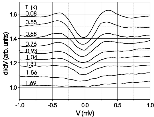
FIG. 3. Tunneling conductance as a function of bias, measured at different temperatures showing that the low-bias suppression of the conductance disappears above T_c (curves are offset for clarity).
