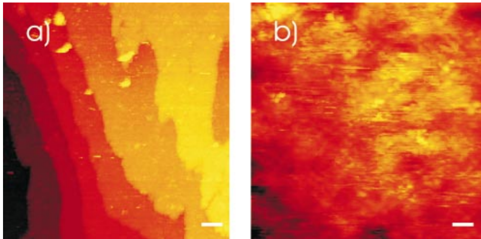
FIG. 1. (Color) Unfiltered images of an in-air cleaved \text{Sr}_2\text{RuO}_4 crystal, taken at 4.2 K. (a) On a larger scale (the white bar is 50 nm long) flat terraces are visible. The terrace height corresponds to the thickness of a unit cell (1.28 nm), within the accuracy of the STM calibration. (b) Although a rather regular structure is visible on a smaller scale (the white bar is 2 nm), no clear atomic resolution has been achieved.
