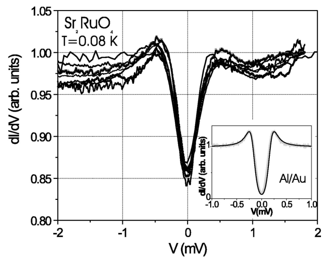
FIG. 2. Tunneling spectra measured at 80 mK on different crystals or at different locations of a same crystal ( dI/dV is normalized to the value at V = 2 mV, for ease of comparison). A \approx 15\% suppression of the conductance at low bias is observed in all curves, demonstrating the reproducibility of our results. The position of the side lobes varies from 380 to 500 \mu\text{eV} . The inset shows the tunneling conductance of an Al tip on Au substrate (thick gray line) and its fit according to BCS theory (black line), from which we infer an effective electron temperature of 500 mK (larger than the crystal temperature) which sets the energy resolution of our measurements.
